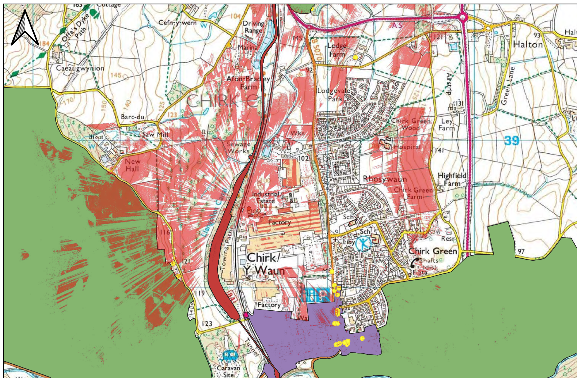
Figure 12. ZTV model - extension 29m height
