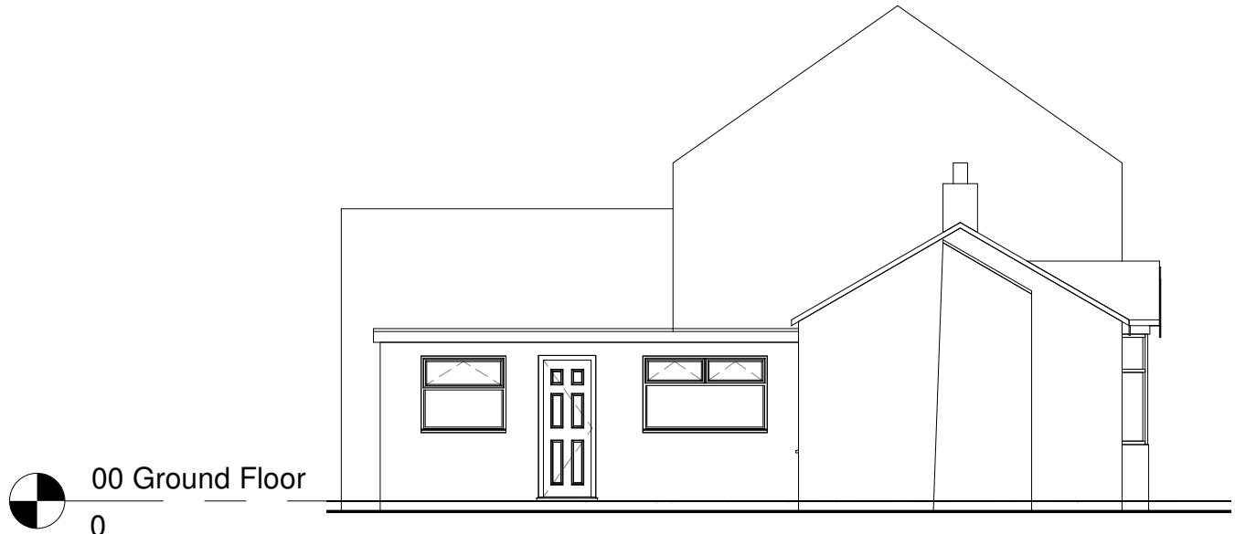
East Elevation 1 : 100
