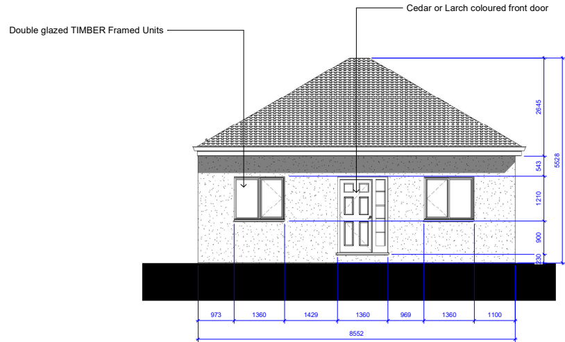
** Proposed Front 1 : 50
