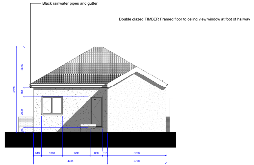
** Proposed Rear 1 : 50
