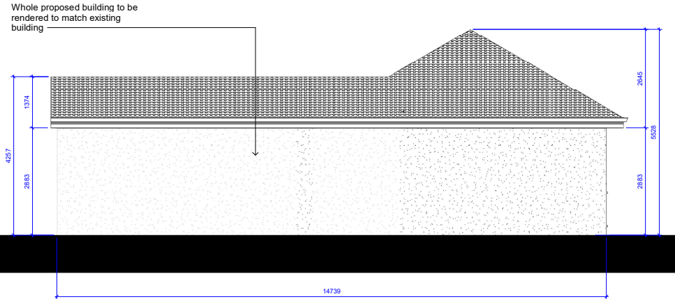
** Proposed Left 1 : 50
