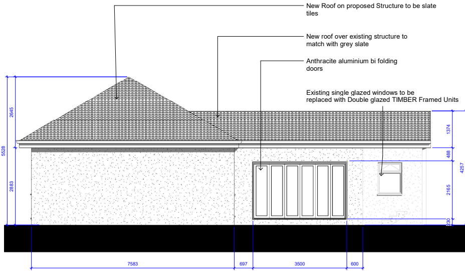
** Proposed Right 1 : 50
