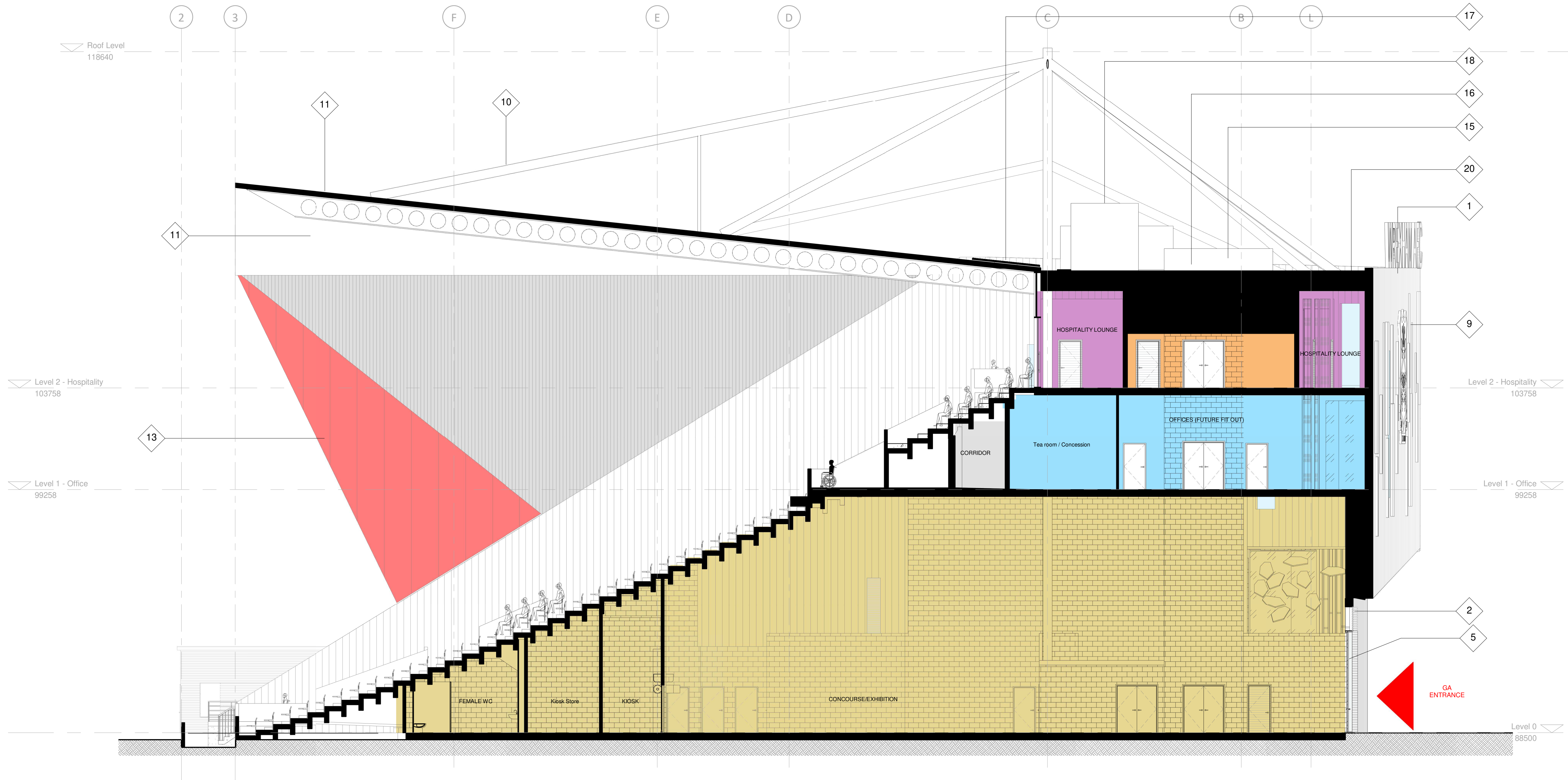
1 Cross Section - Seated Accomodation 1 : 100
