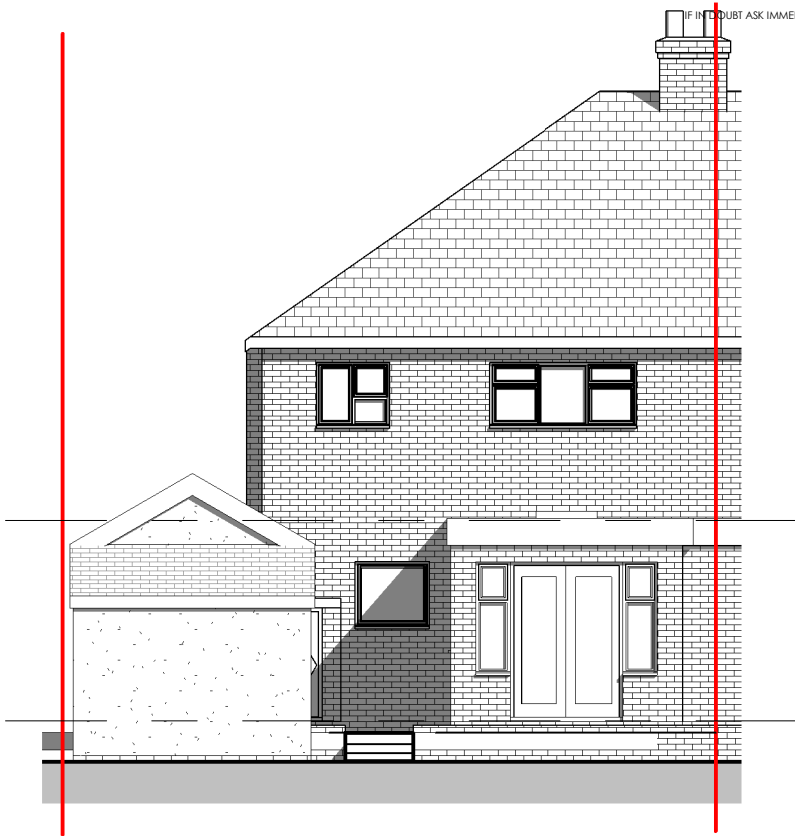
Rear Elevation 1 : 100
