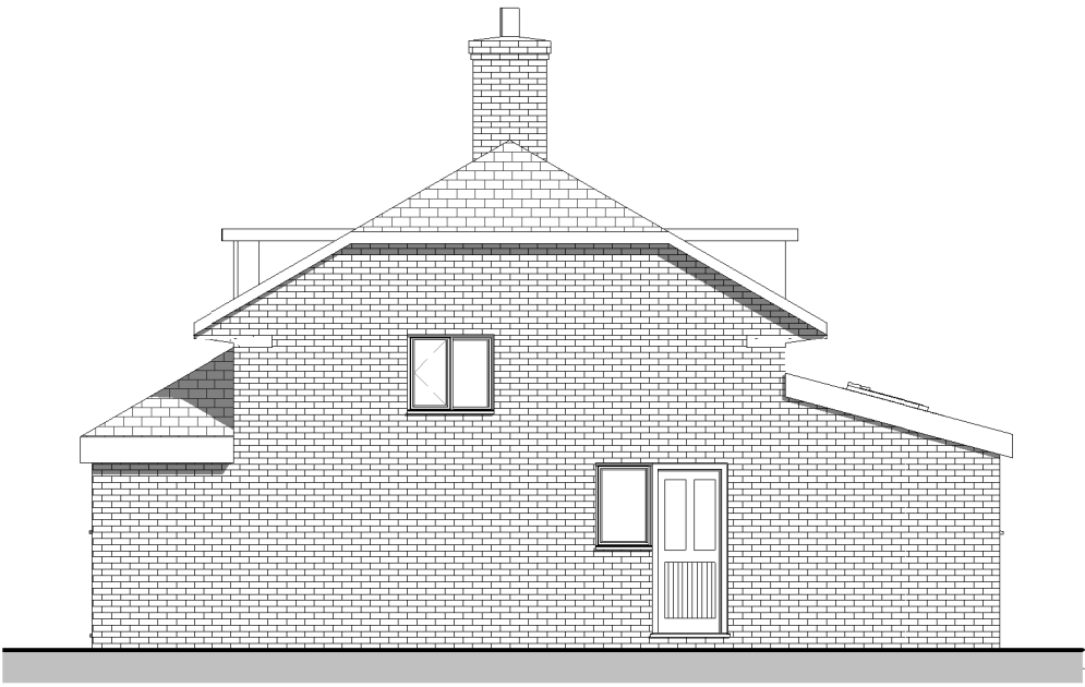
Side Elevation 1 : 100
