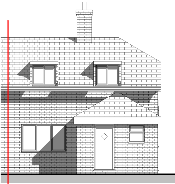
Front Elevation 1 : 100
