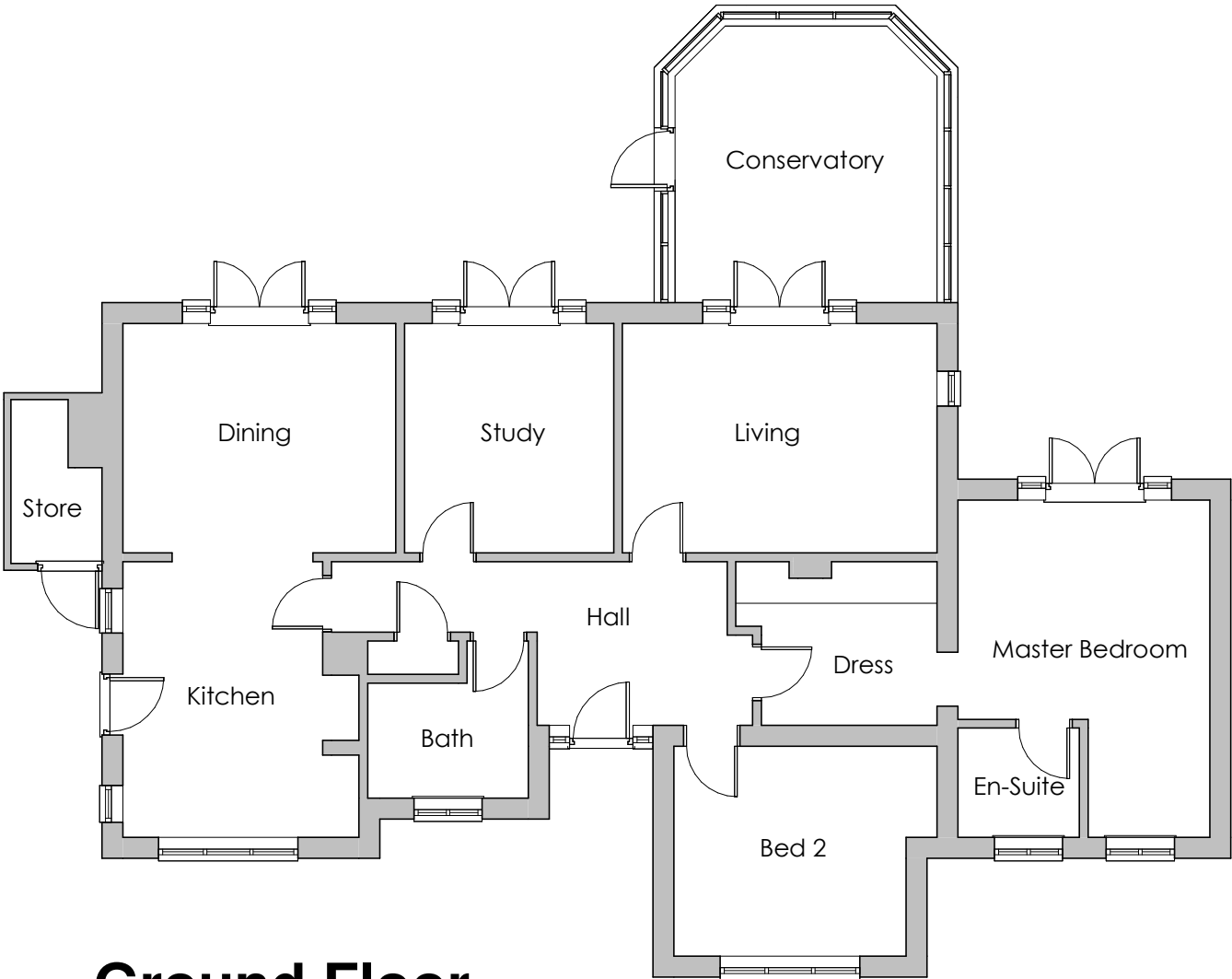
Ground Floor 1 : 100
