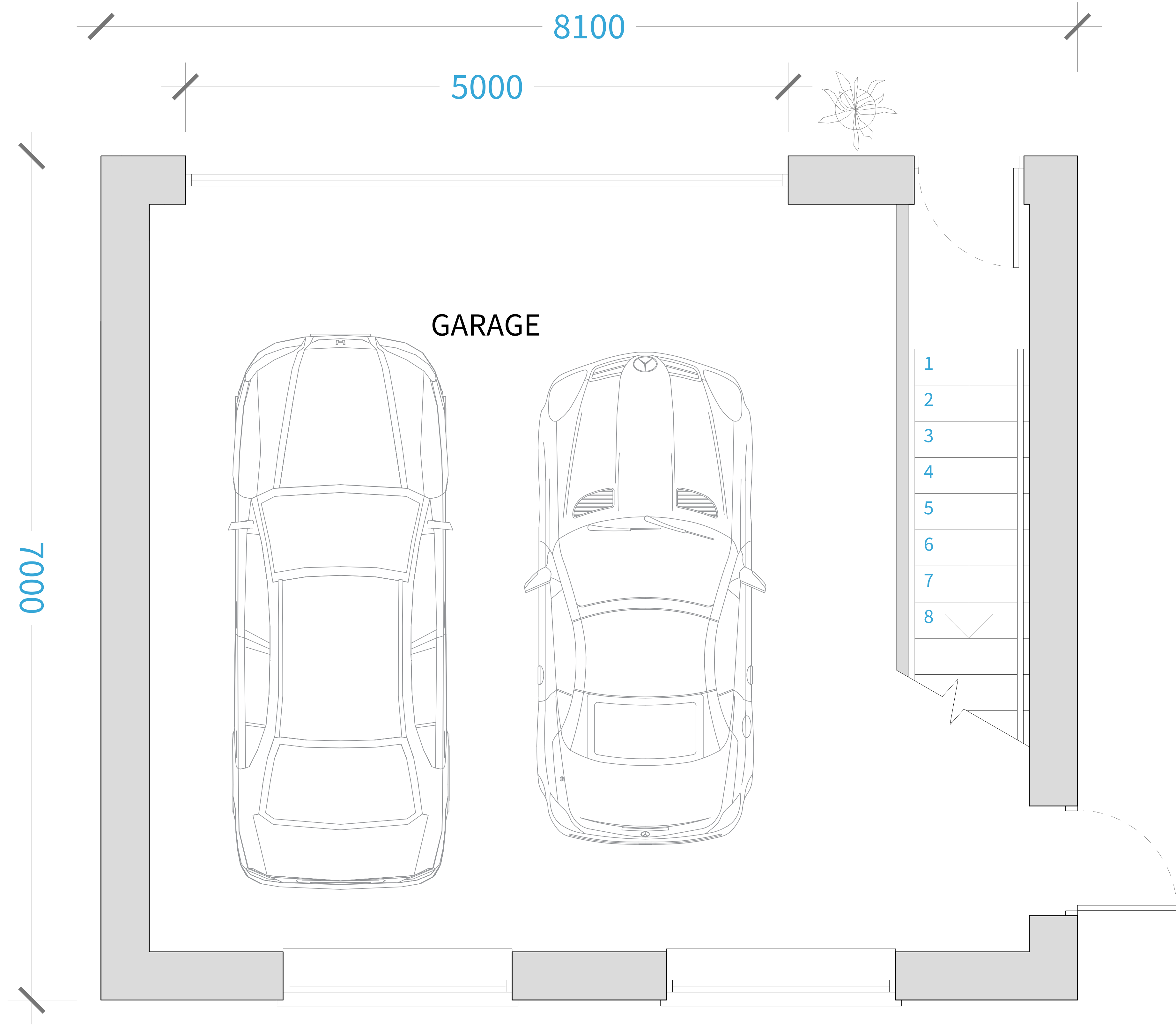
PROPOSED GROUND FLOOR (1:20)
