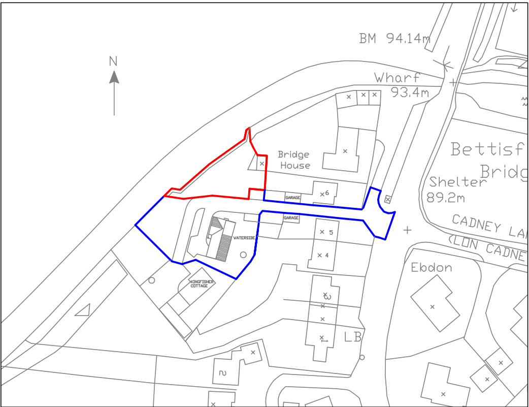
LOCATION PLAN 1:1250
