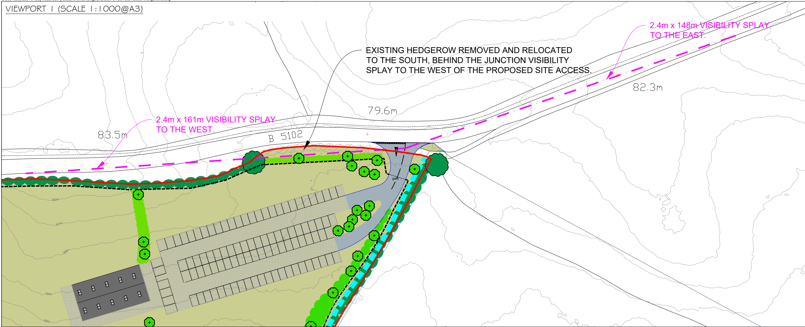
VIEWPORT 2 (SCALE 1:500@A3)
