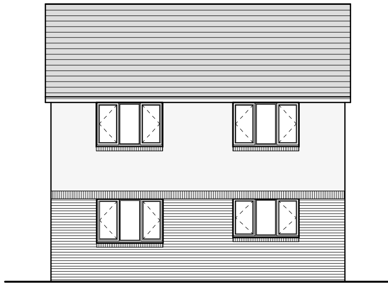
Rear Elevation 1:100
