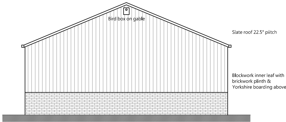
PROPOSED SOUTH EAST ELEVATION
