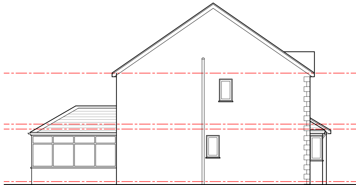
Side-01 Elevation 1:100
