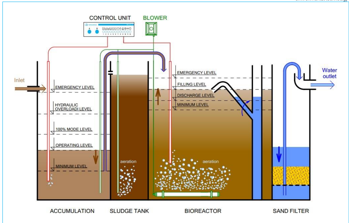
Figure no. 4: Flow (nitrification) stage – drawing water out of the activation tank (decanting)
