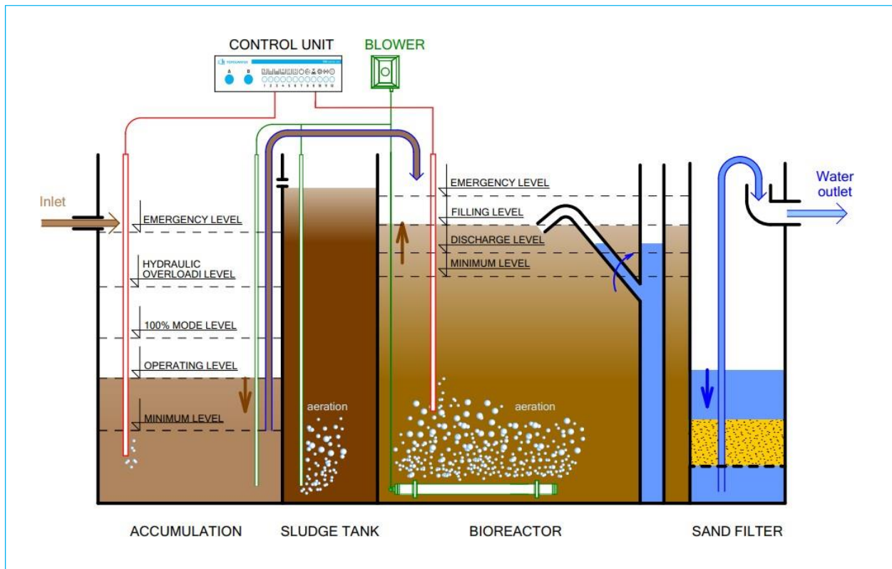
Figure no. 3: Flow (nitrification) stage – filling of the activation tank (bioreactor)
