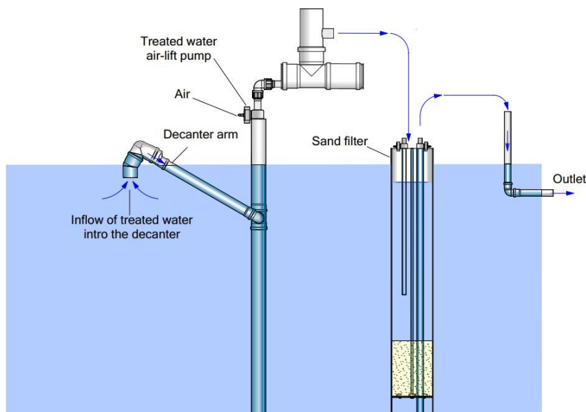
Figure no. 2: Principle of the decanter functioning
