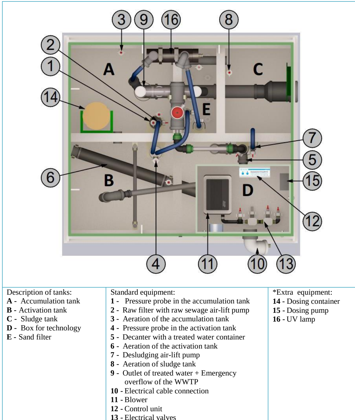
Figure no. 1: Ground plan of TOPAS
