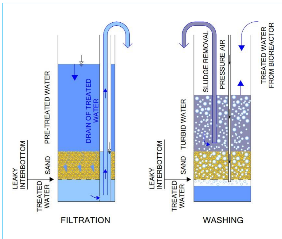
Figure no. 5: Technological diagram of the sand filter functioning
