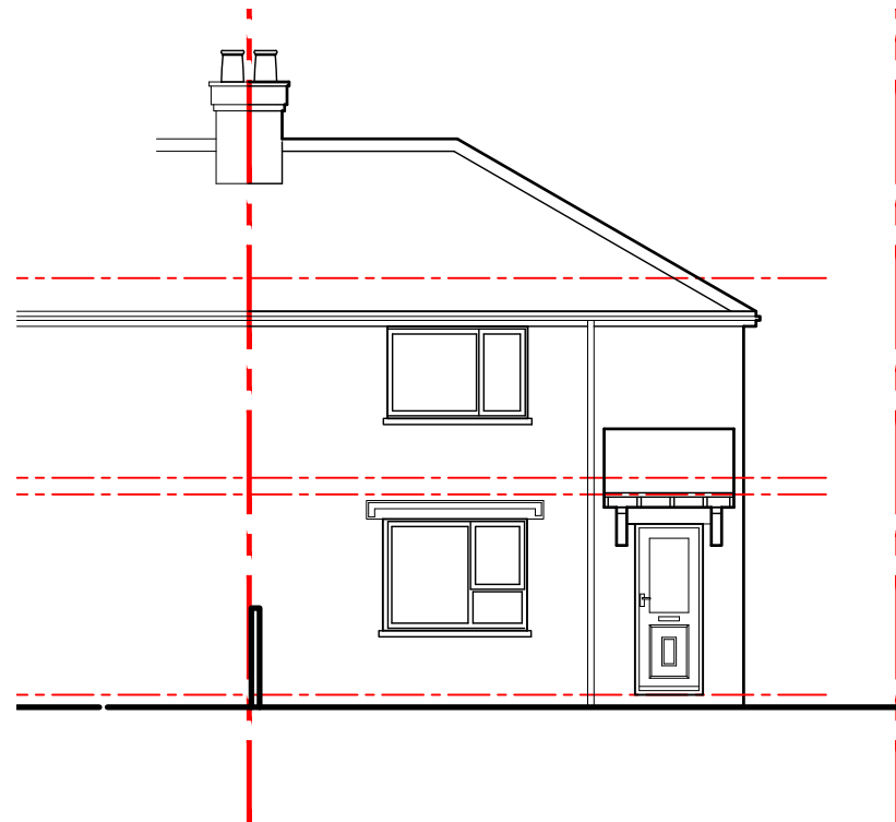
Front elevation 1:100
