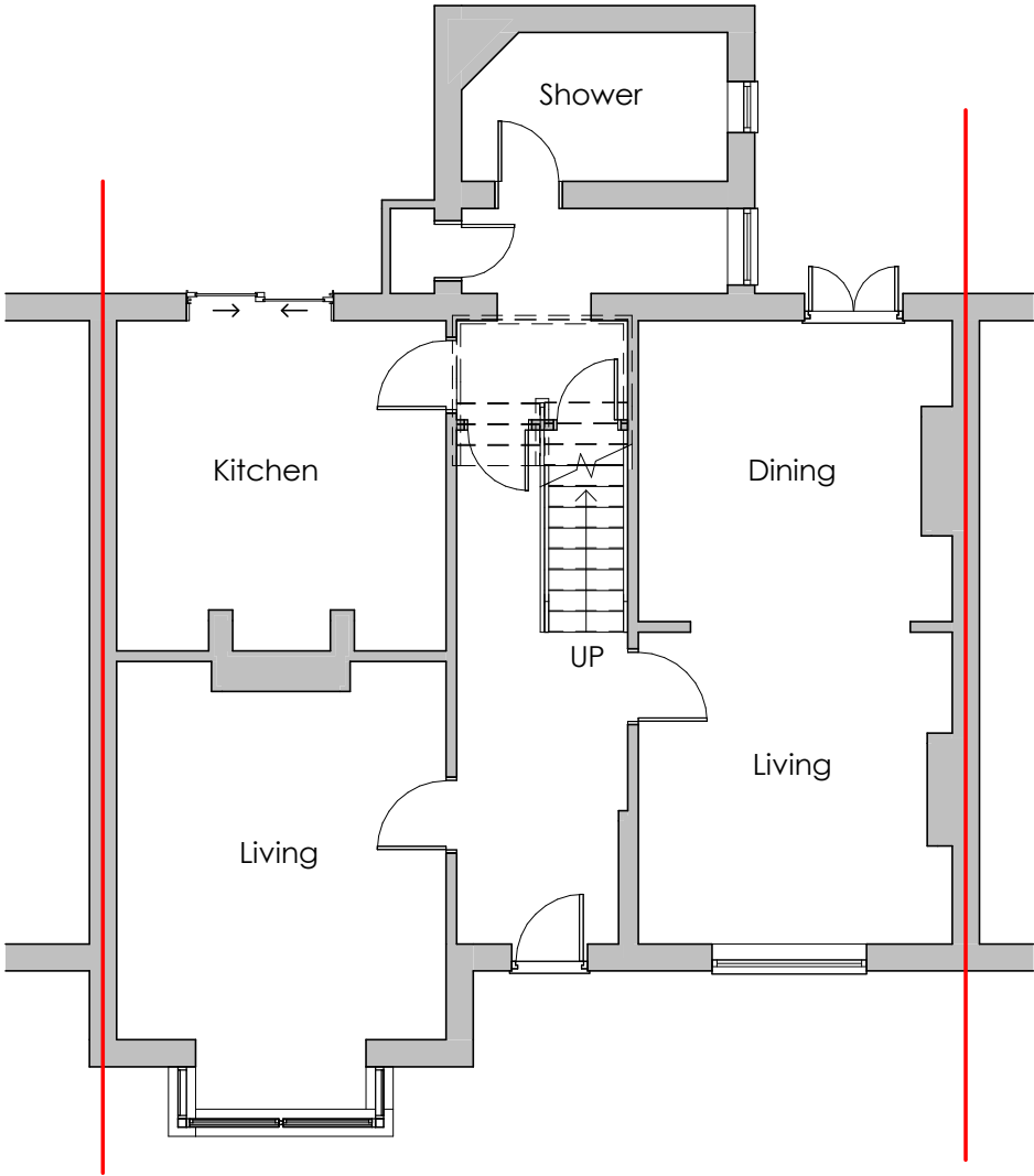
Ground Floor 1 : 100
