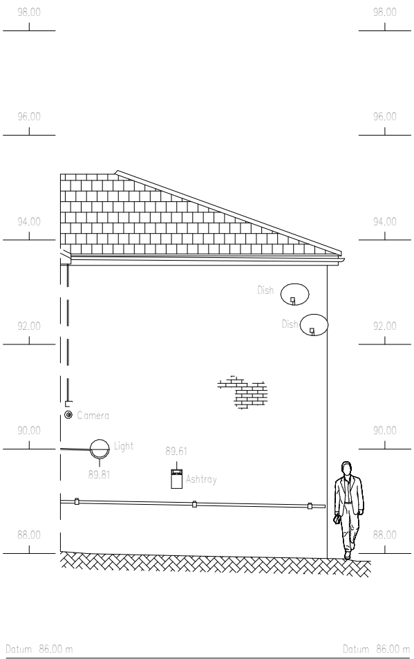
Elevation H
