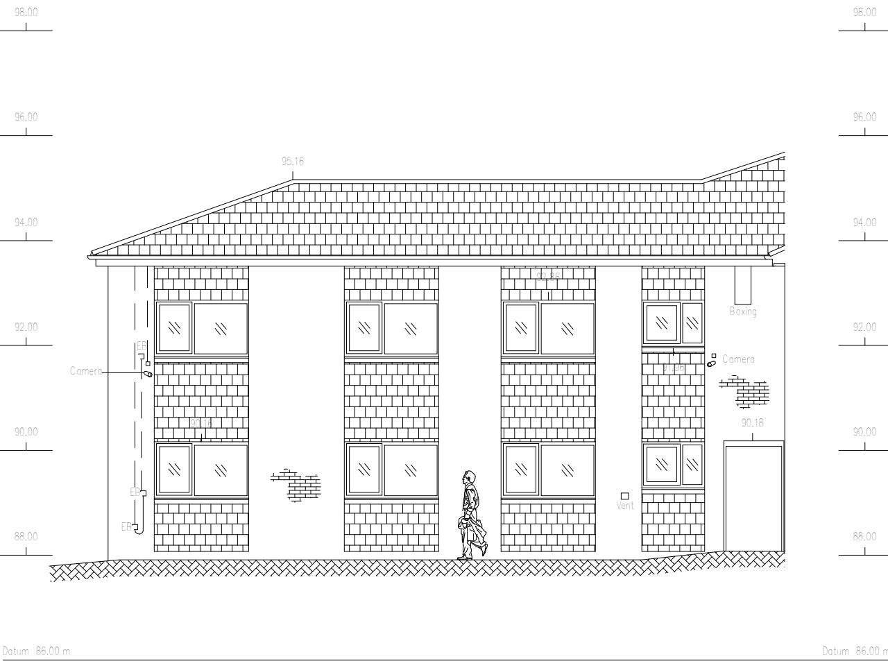
Elevation K
