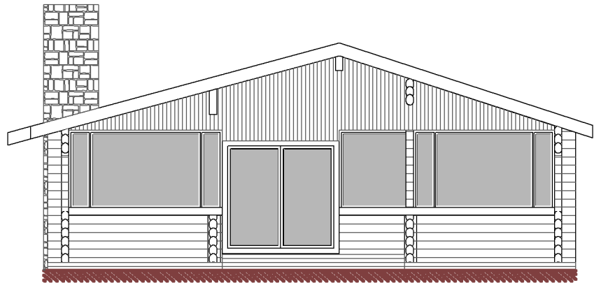
Front Elevation
