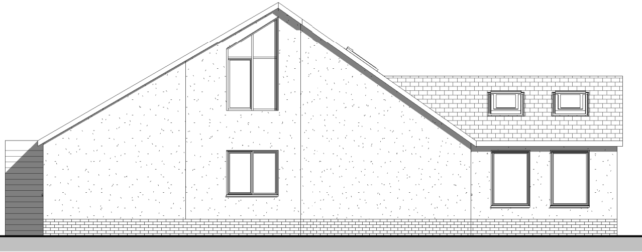
Side Elevation 1 : 100
