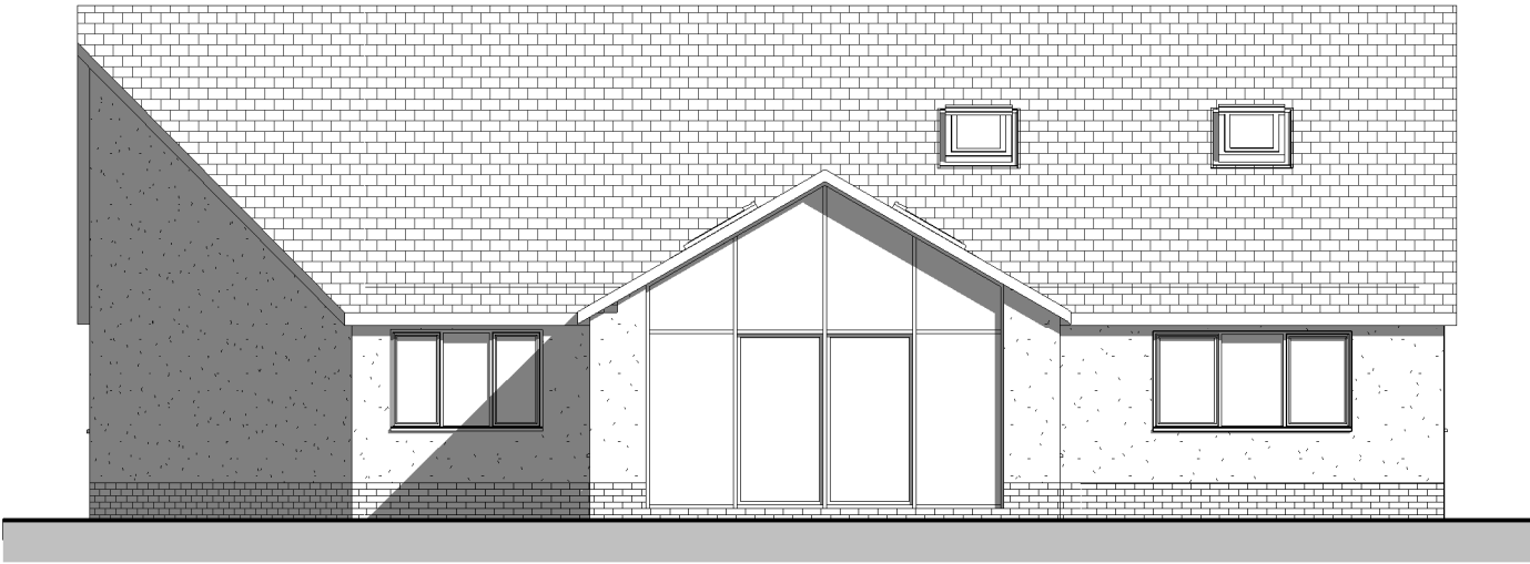
Rear Elevation 1 : 100
