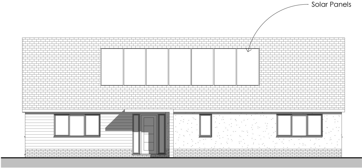
Front Elevation 1 : 100
