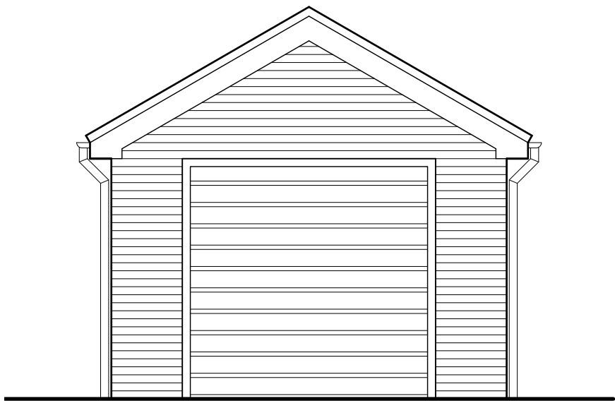
Front elevation 1:50
