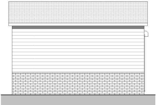
Side Elevation 1 : 100
