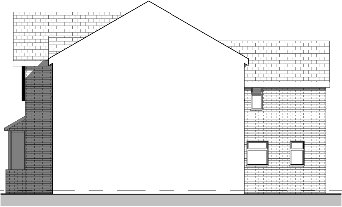
Side Elevation 1 : 100
