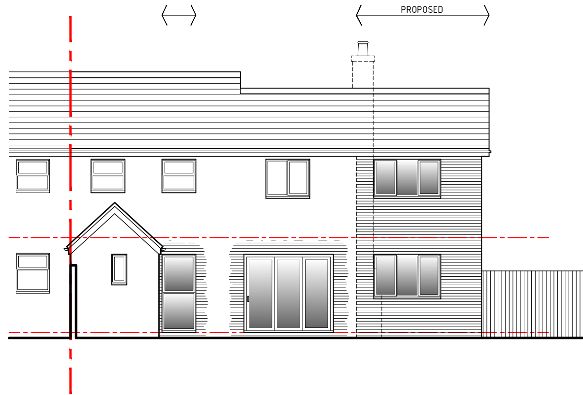
Rear elevation 1:100
