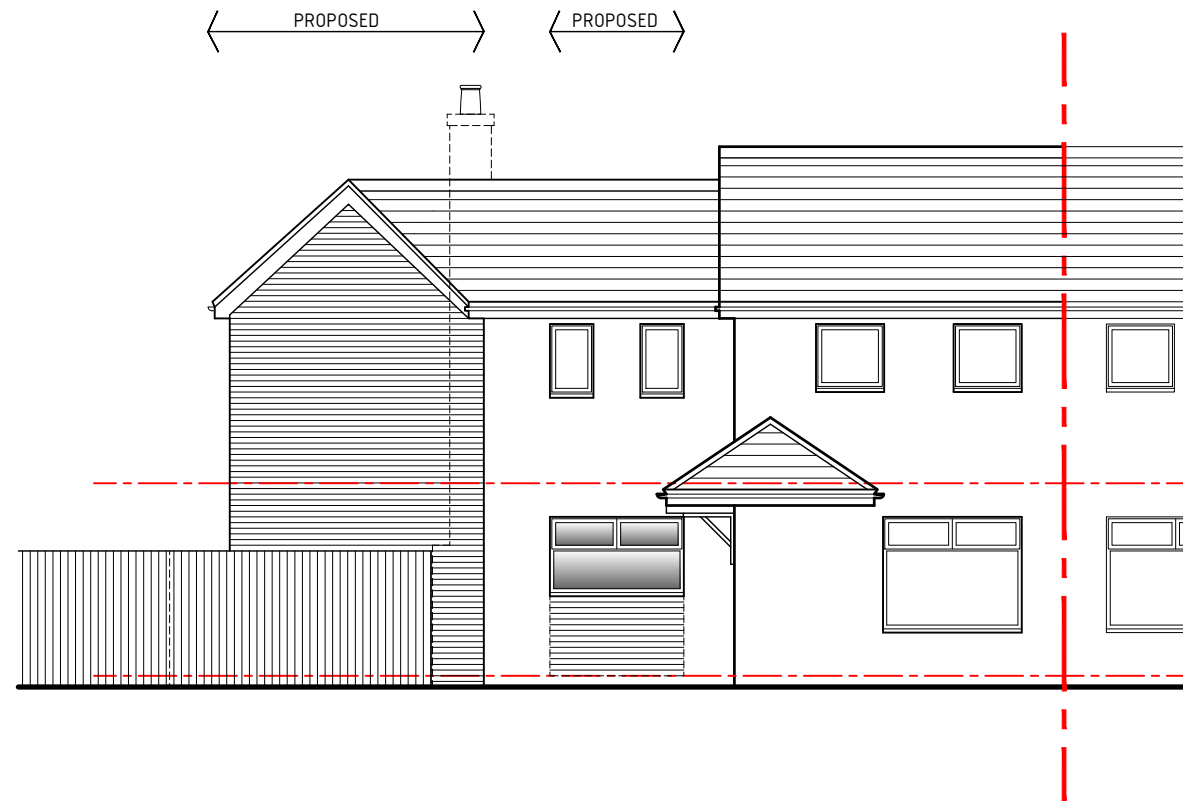
Front elevation 1:100
