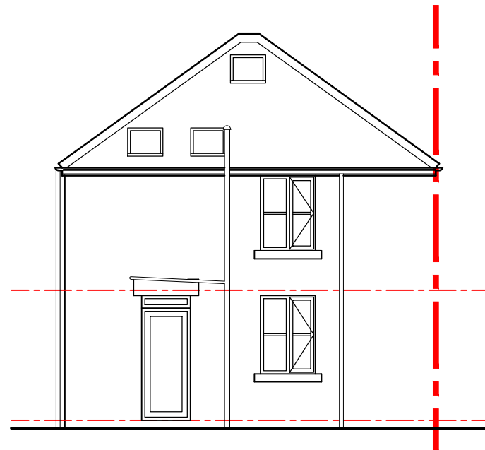
Rear Elevation
