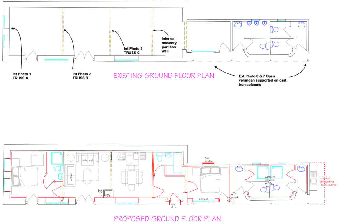
The Engine House. Scale : 1:75 @ A3
