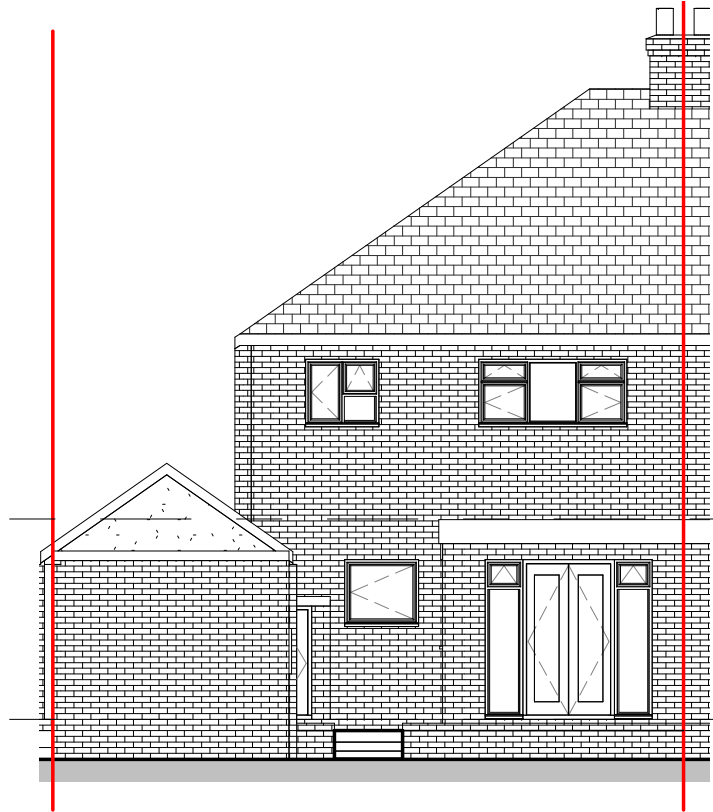
Rear Elevation 1 : 100
