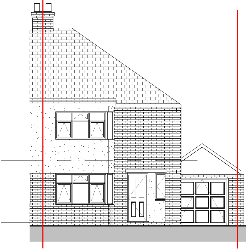
Front Elevation 1 : 100
