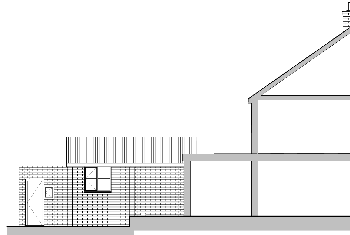
Side Elevation 1 : 100
