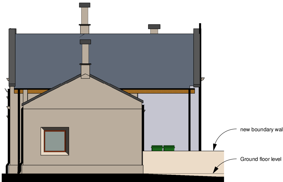
East Elevation Proposed
