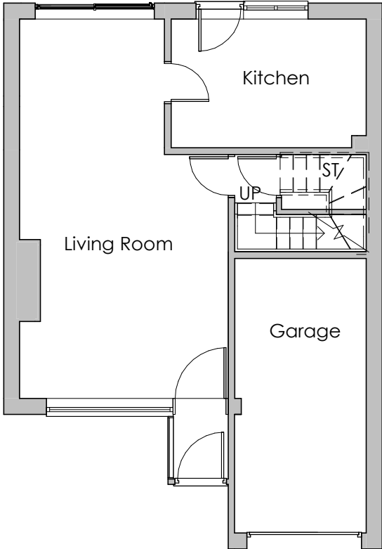
Ground Floor 1 : 100
