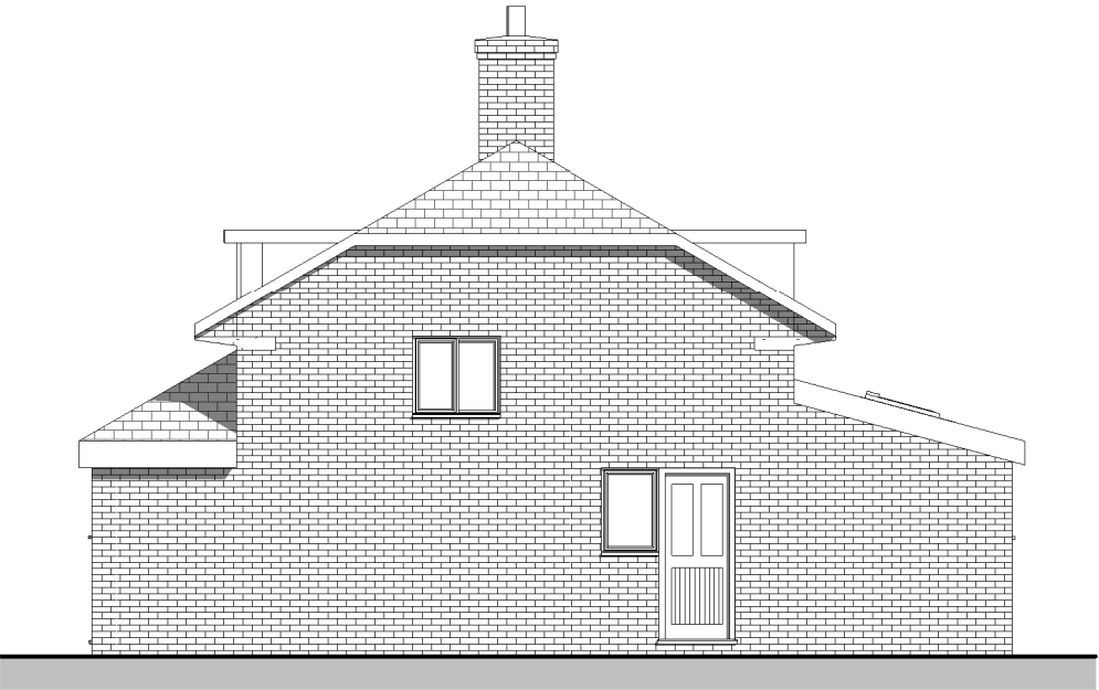
Side Elevation 1 : 100
