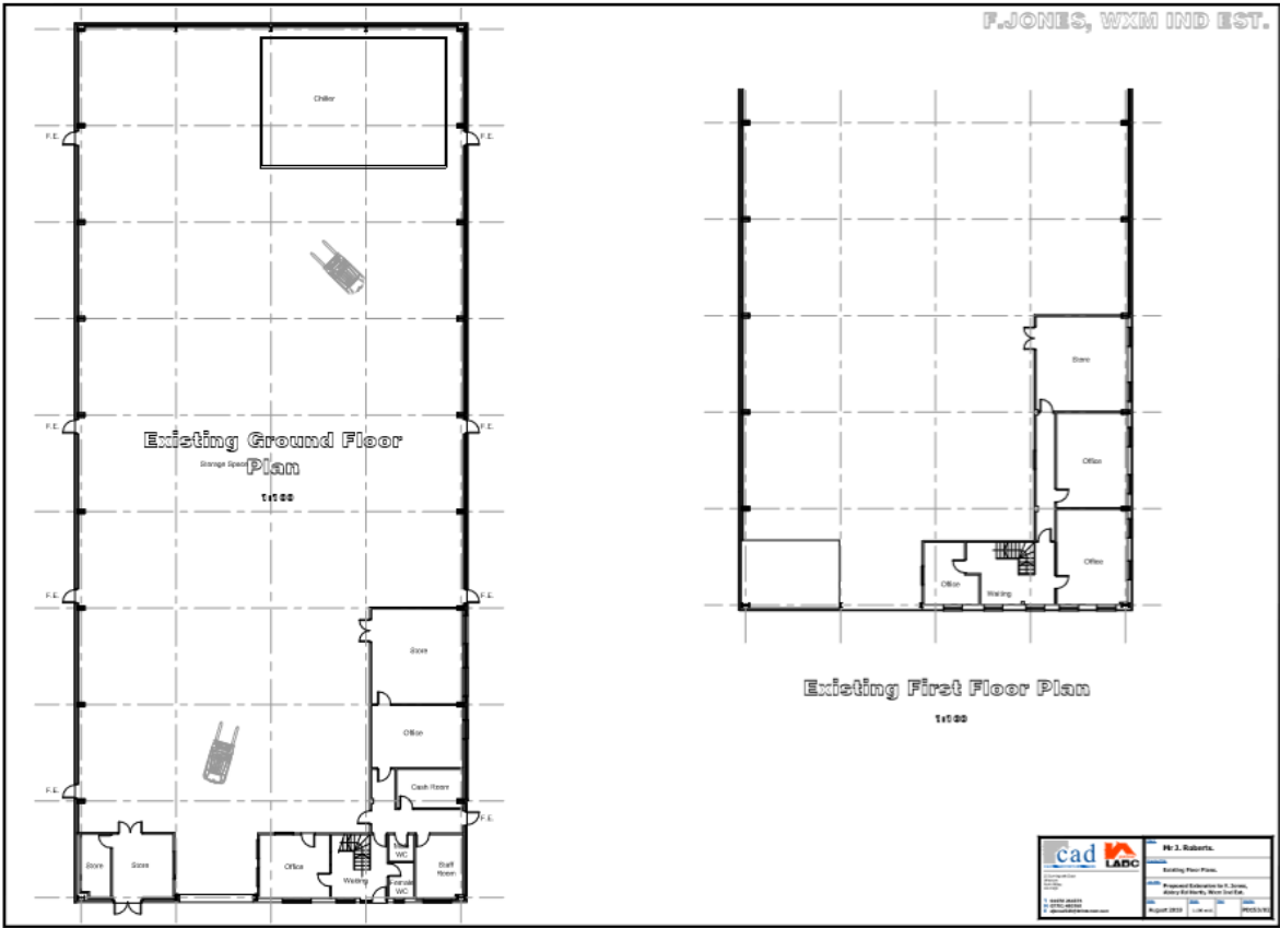
Drawing 5 – Existing floor plan
