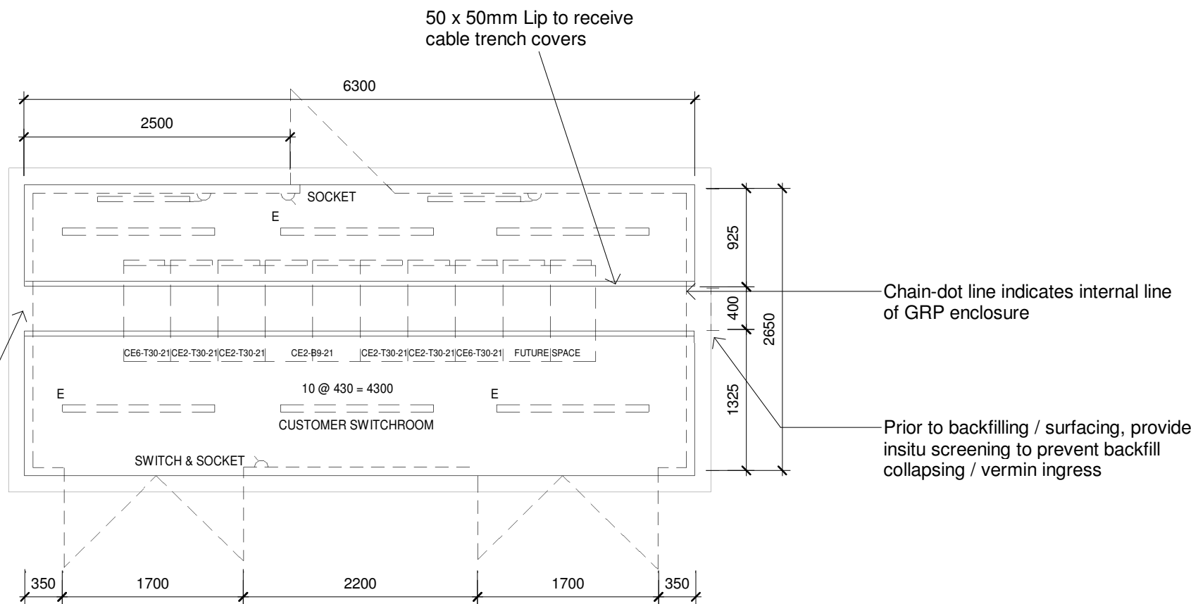
Switchroom Layout 1 : 50
