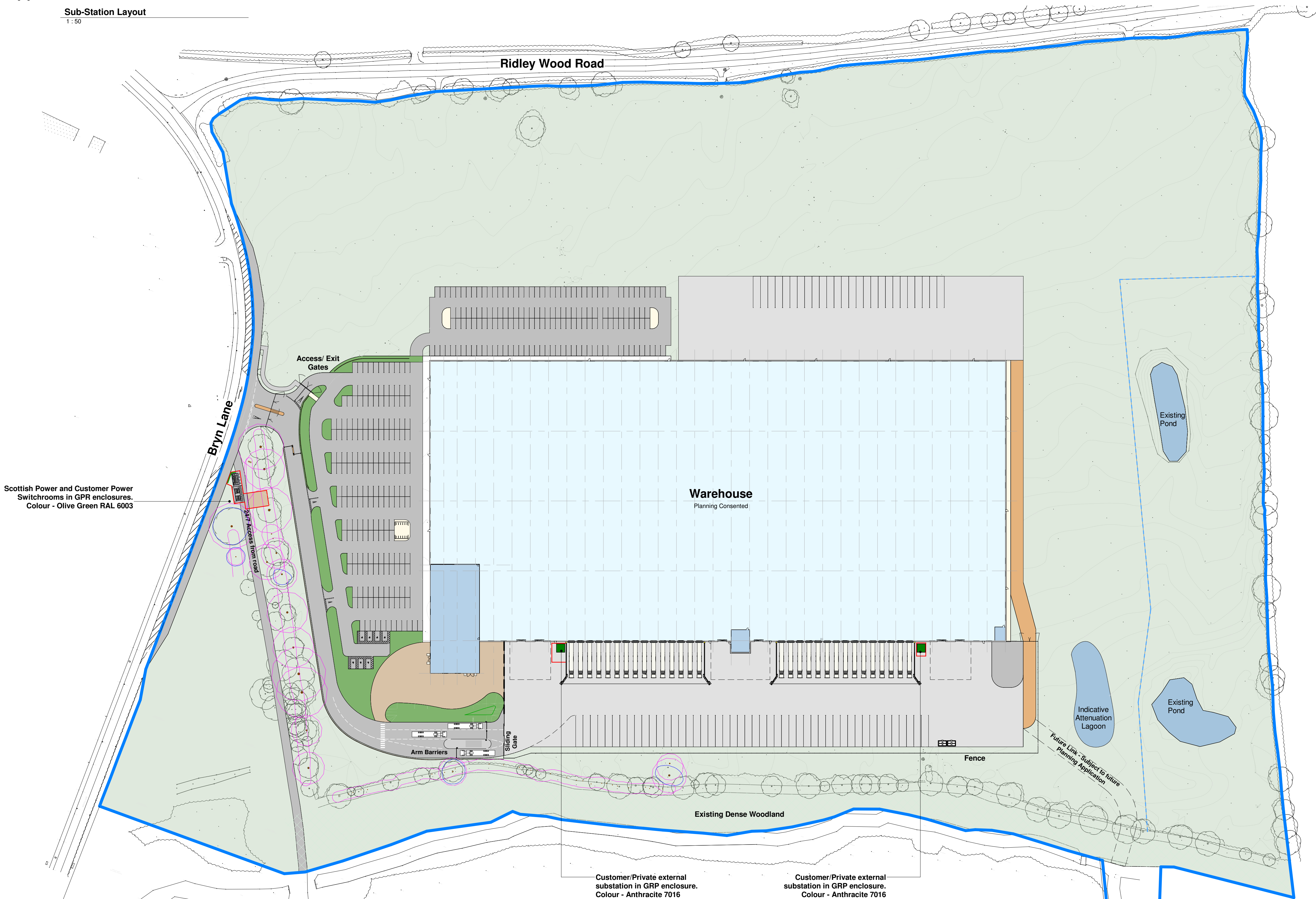
05-ZZ Proposed Sub Station Location Plan 1 : 1000
