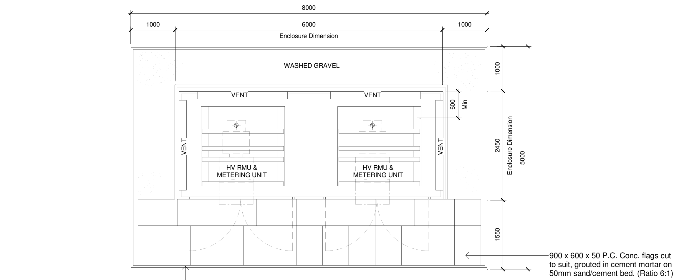
Sub-Station Layout 1 : 50
