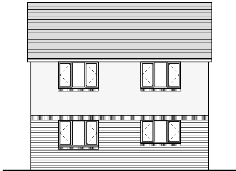
Rear Elevation 1:100
