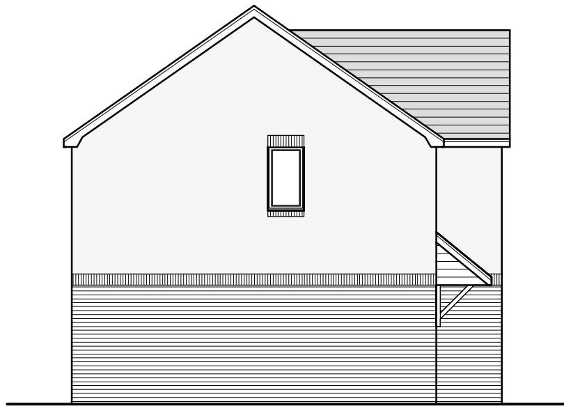
Side Elevation 1:100
