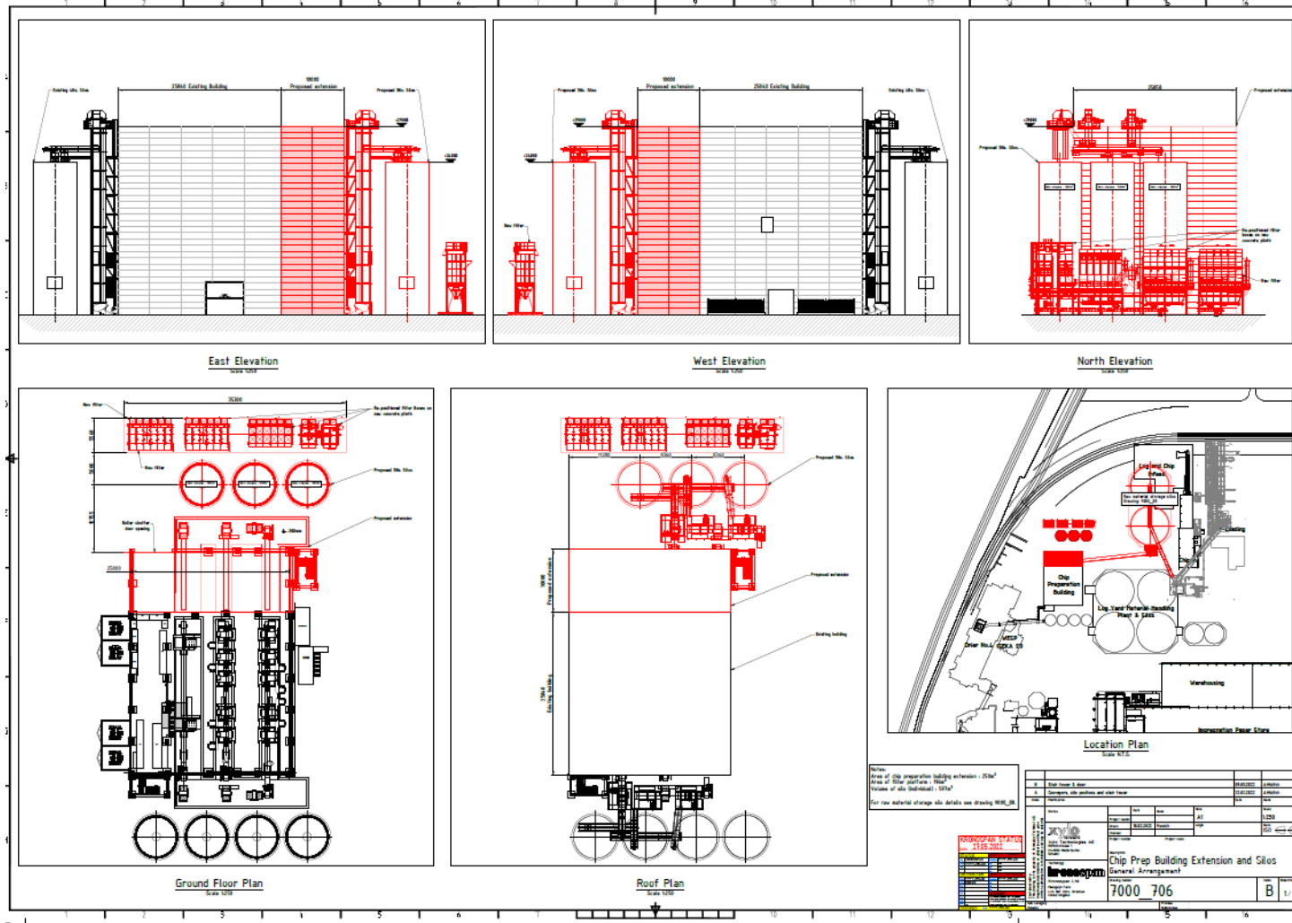
Figure 2: Layout of Proposed Development
