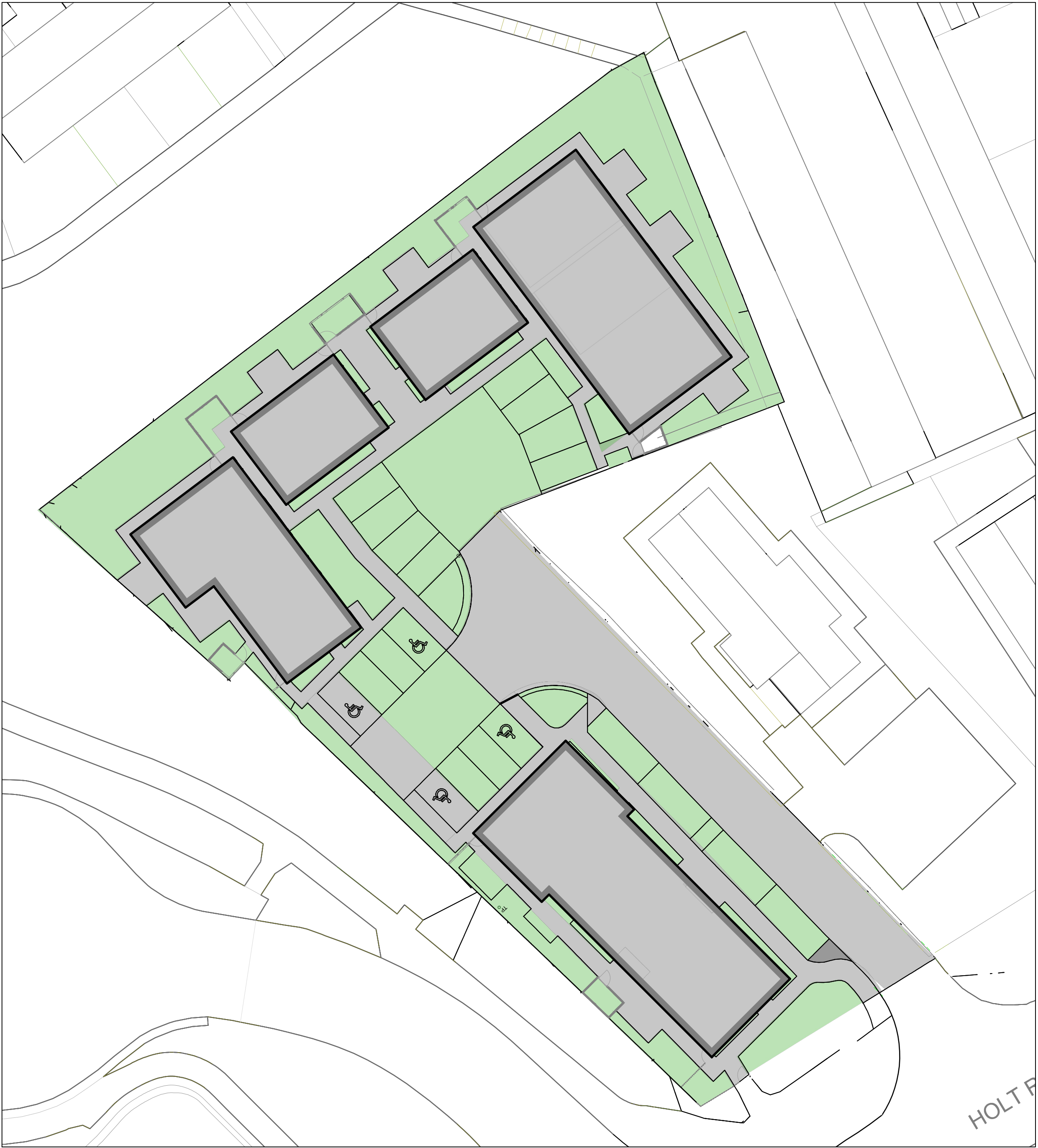
PROPOSED PERMEABLE AND IMPERMEABLE AREAS 1:250
