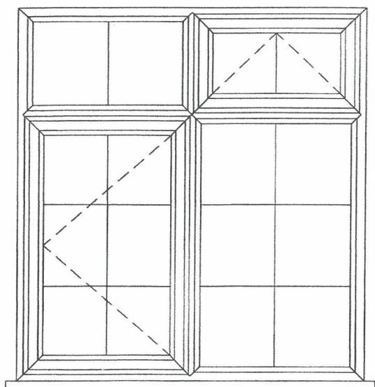
STANDARD CASEMENT (Georgian Inserts)
