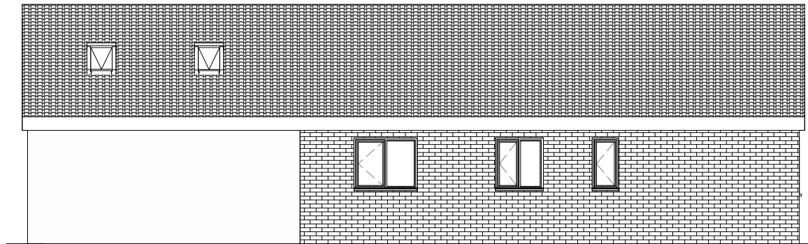
3 Proposed East 1 : 100
