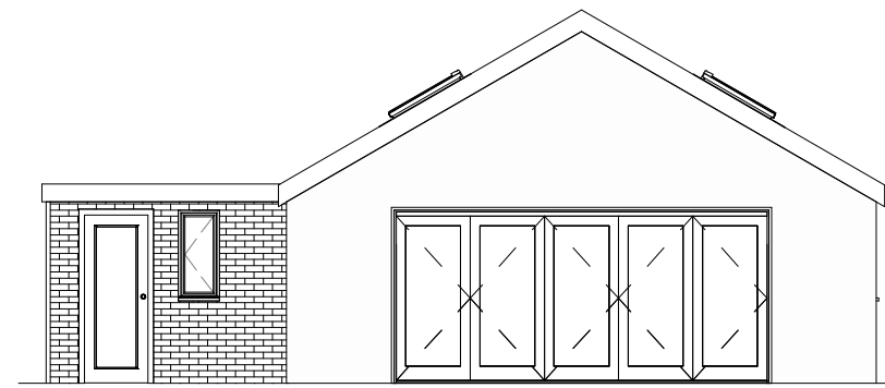
2 Proposed South 1 : 100
