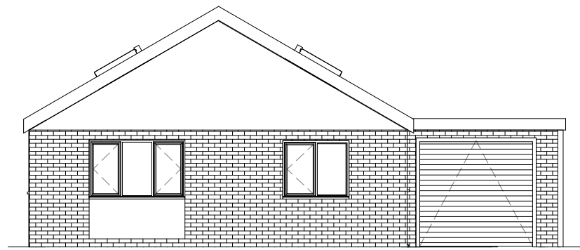
1 Proposed North 1 : 100
