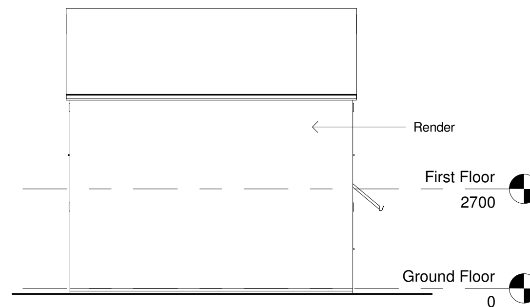
East Elevation 1 : 100
