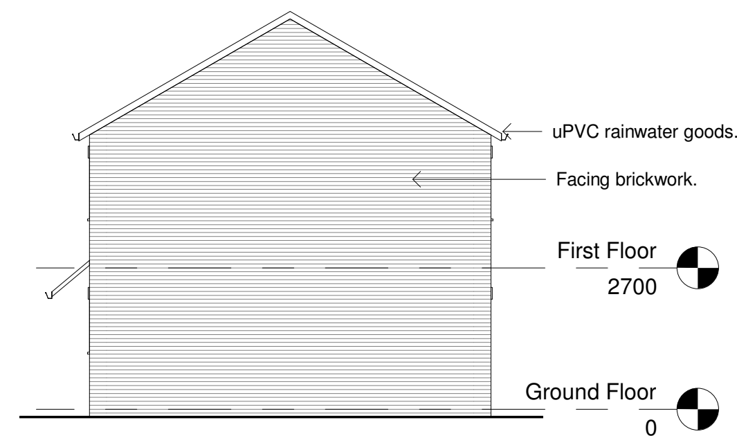
East Elevation 1 : 100
