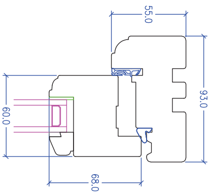
Window Head Rail
