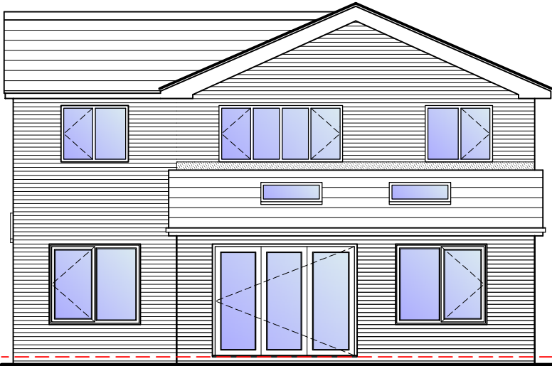
REAR ELEVATION
