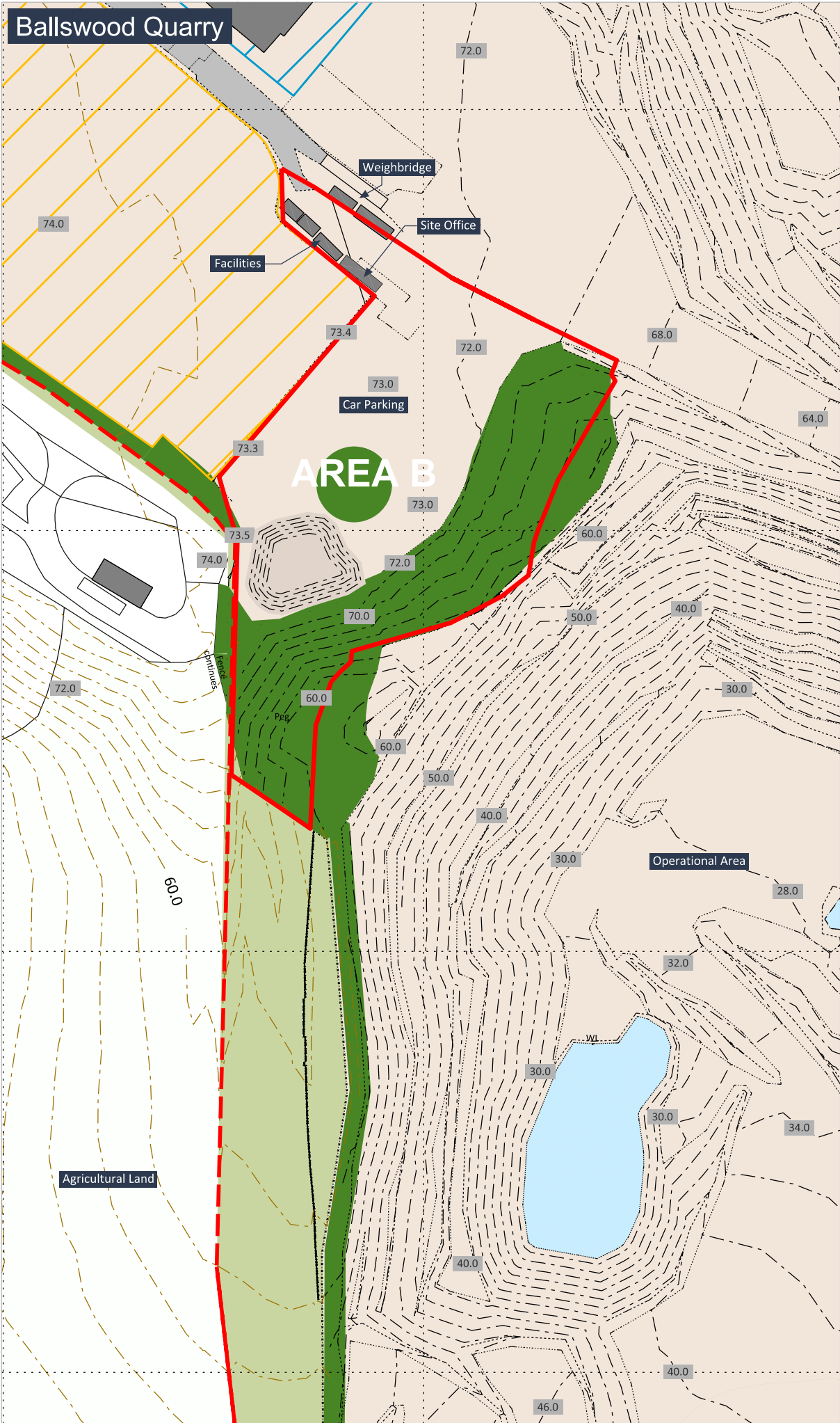
AREA B Current Topographic Survey (June 2022) - 1:1,250 @A3
