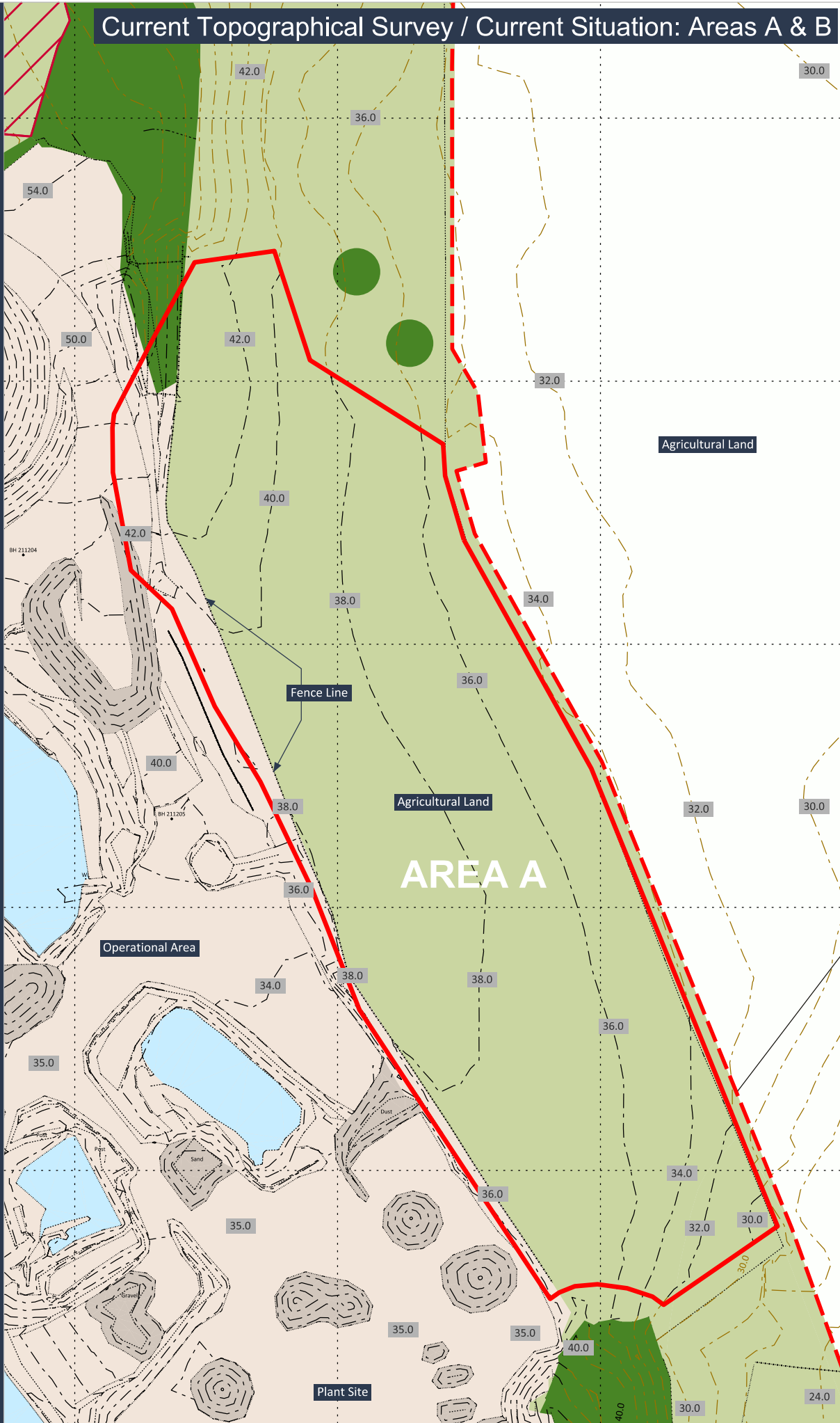
AREA A Current Topographic Survey (June 2022) - 1:2,000 @A3
