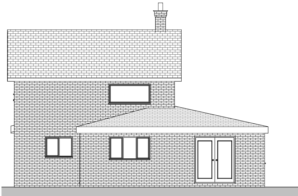
Rear Elevation 1 : 100
