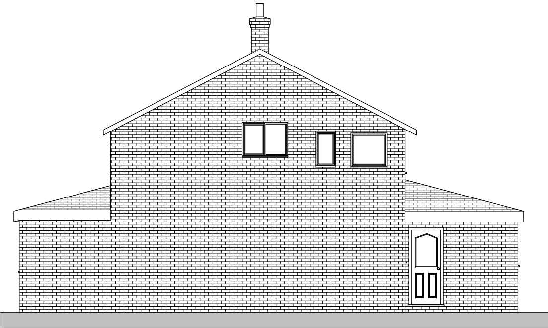
Side Elevation 1 : 100
