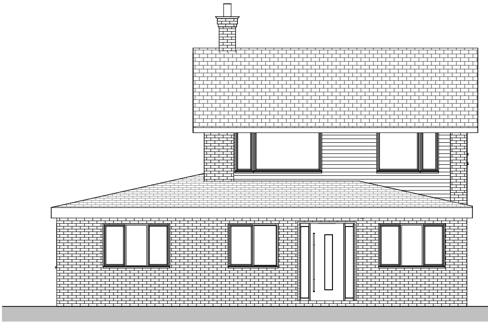
Front Elevation 1 : 100
