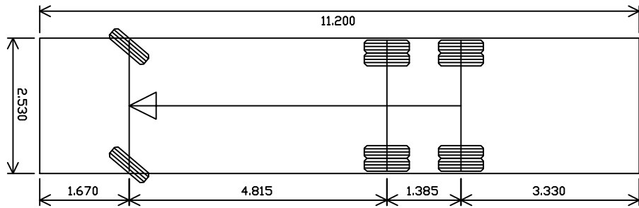
REFUSE VEHICLE
