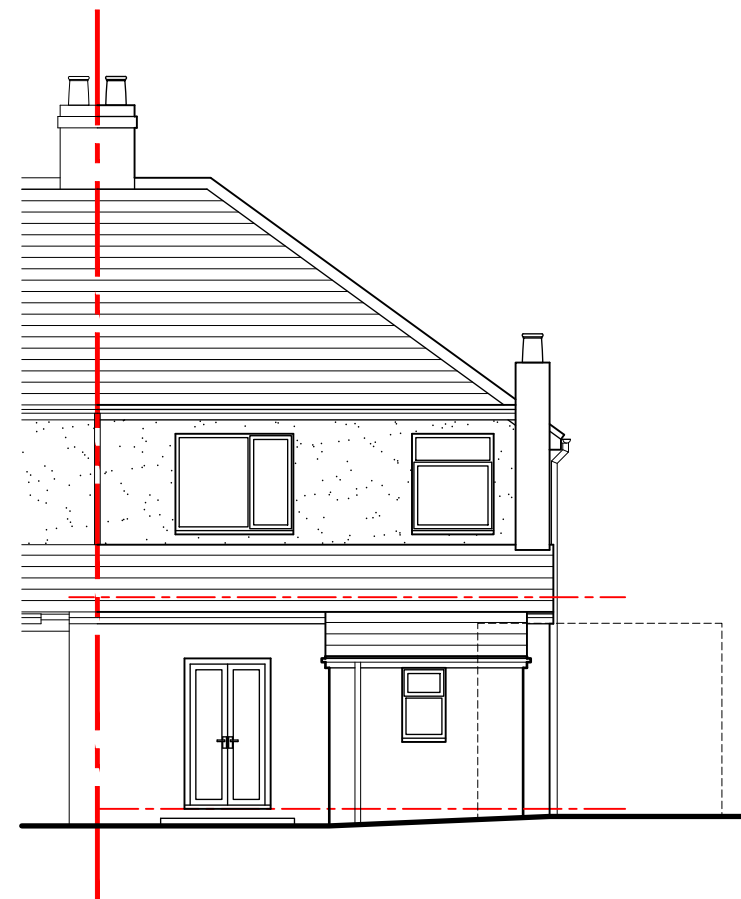
Rear elevation 1:100
