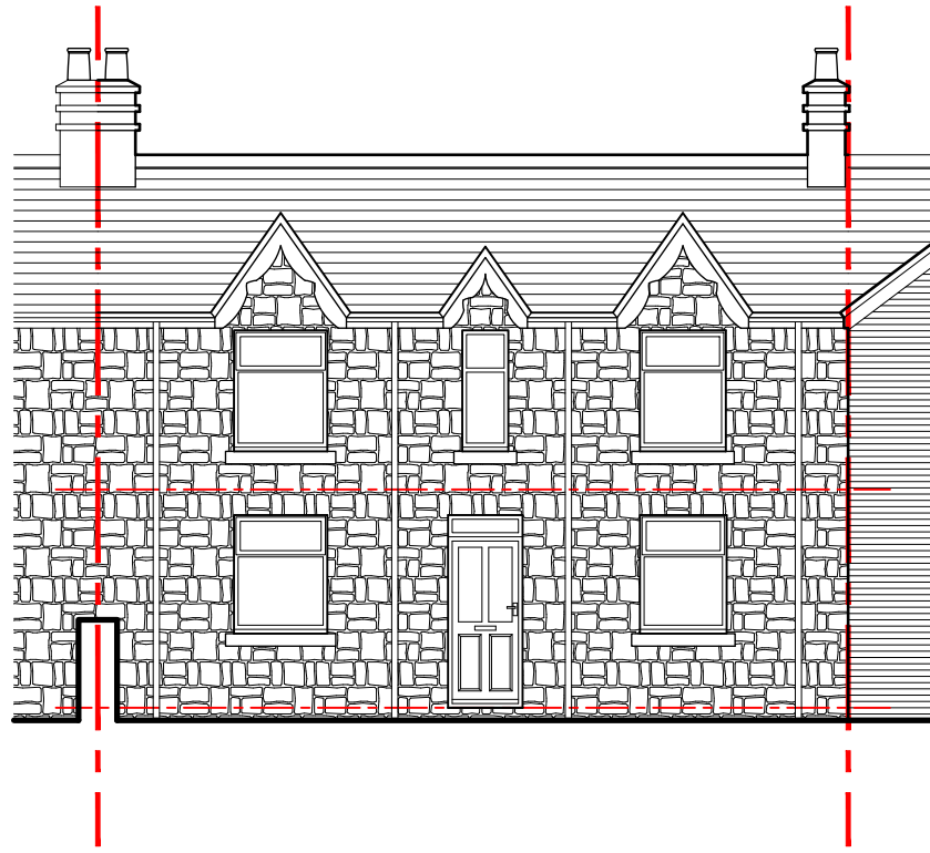
Front Elevation 1:100
