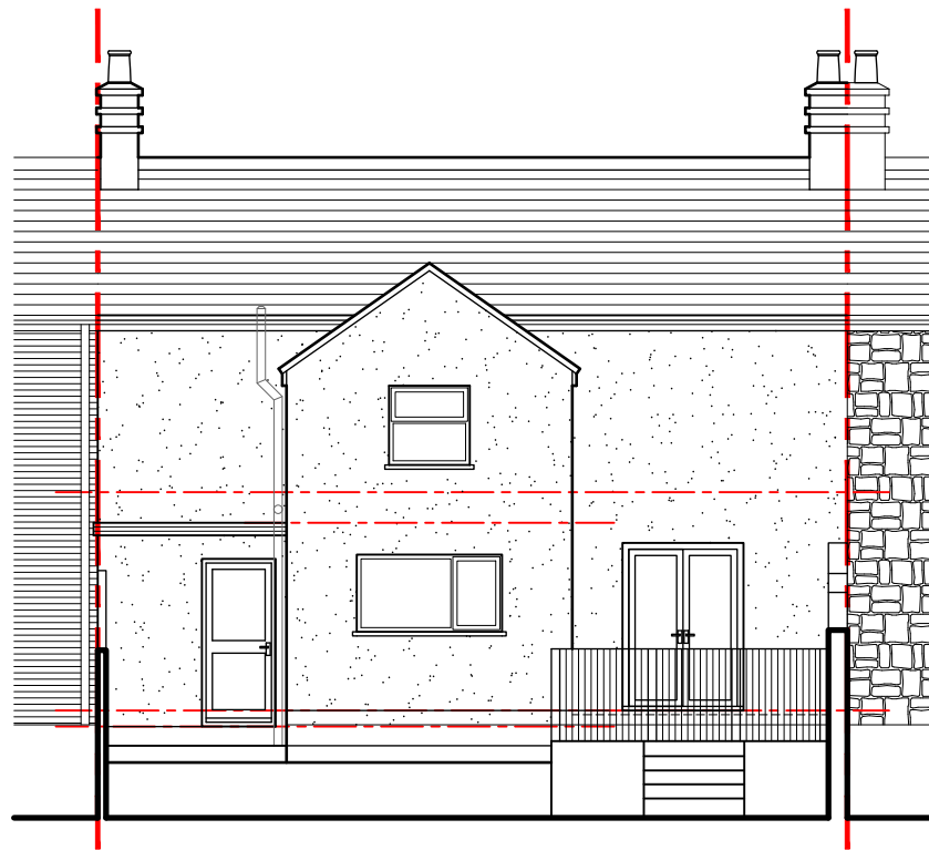
Rear Elevation 1:100
