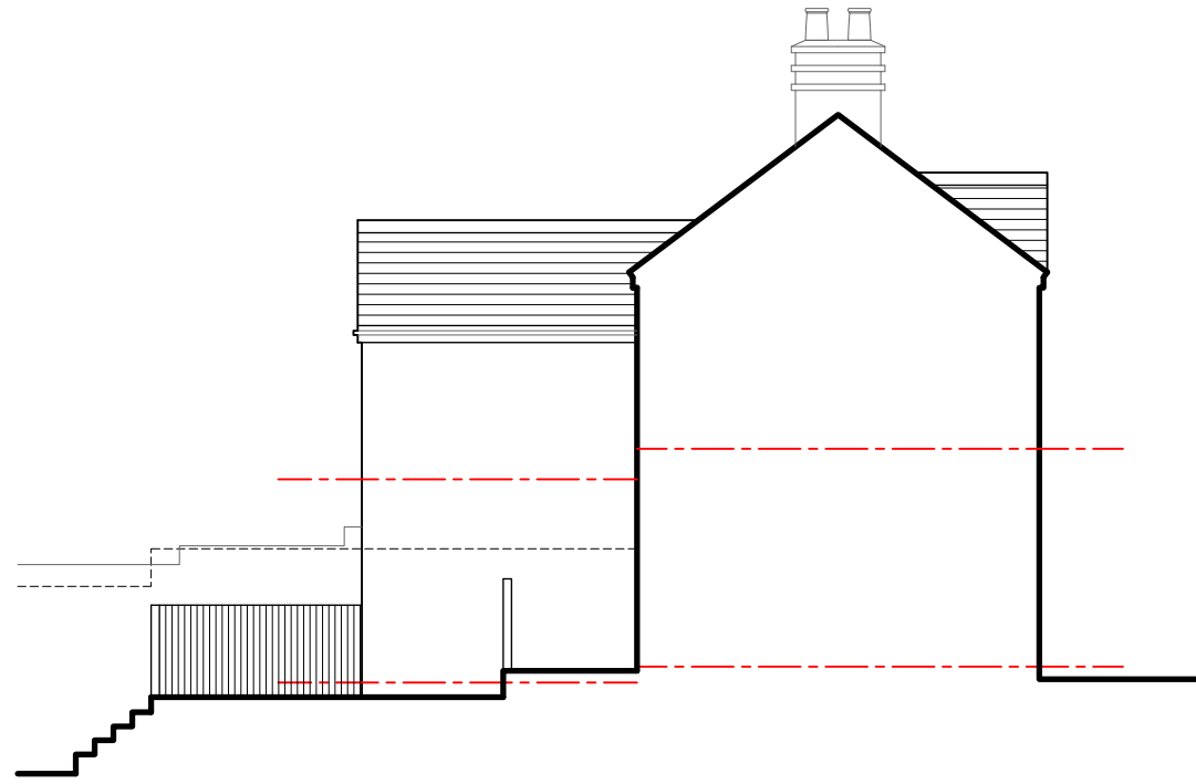
Side-01 Elevation 1:100
