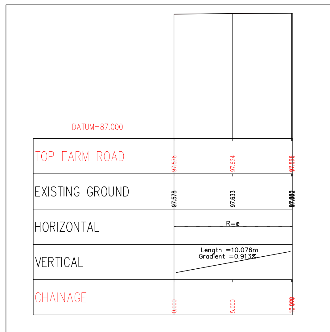
TOP FARM ROAD LONG SECTION @ 1:200 SCALE
