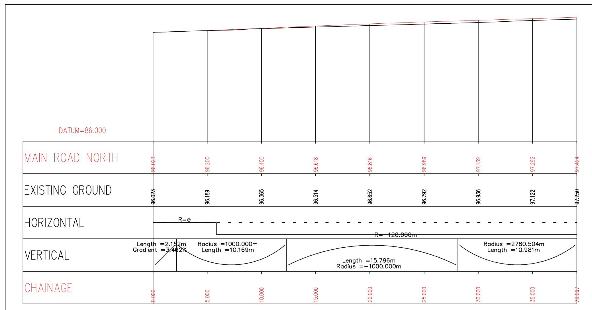
MAIN ROAD (NORTH OF RBT) LONG SECTION @ 1:200 SCALE
