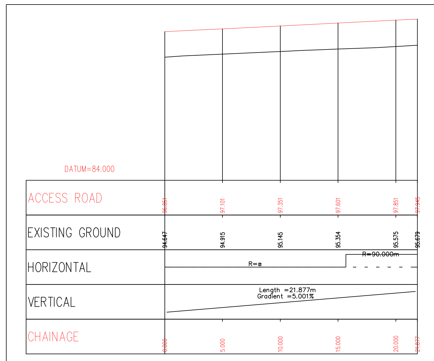
SITE ACCESS ARM LONG SECTION @ 1:200 SCALE
