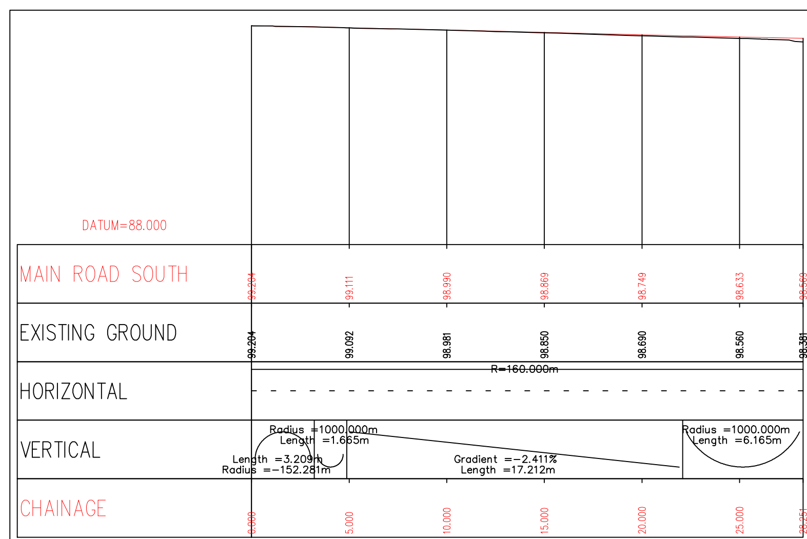
MAIN ROAD (SOUTH OF RBT) LONG SECTION @ 1:200 SCALE
