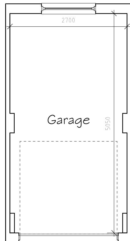
Floor Plan 1:50
