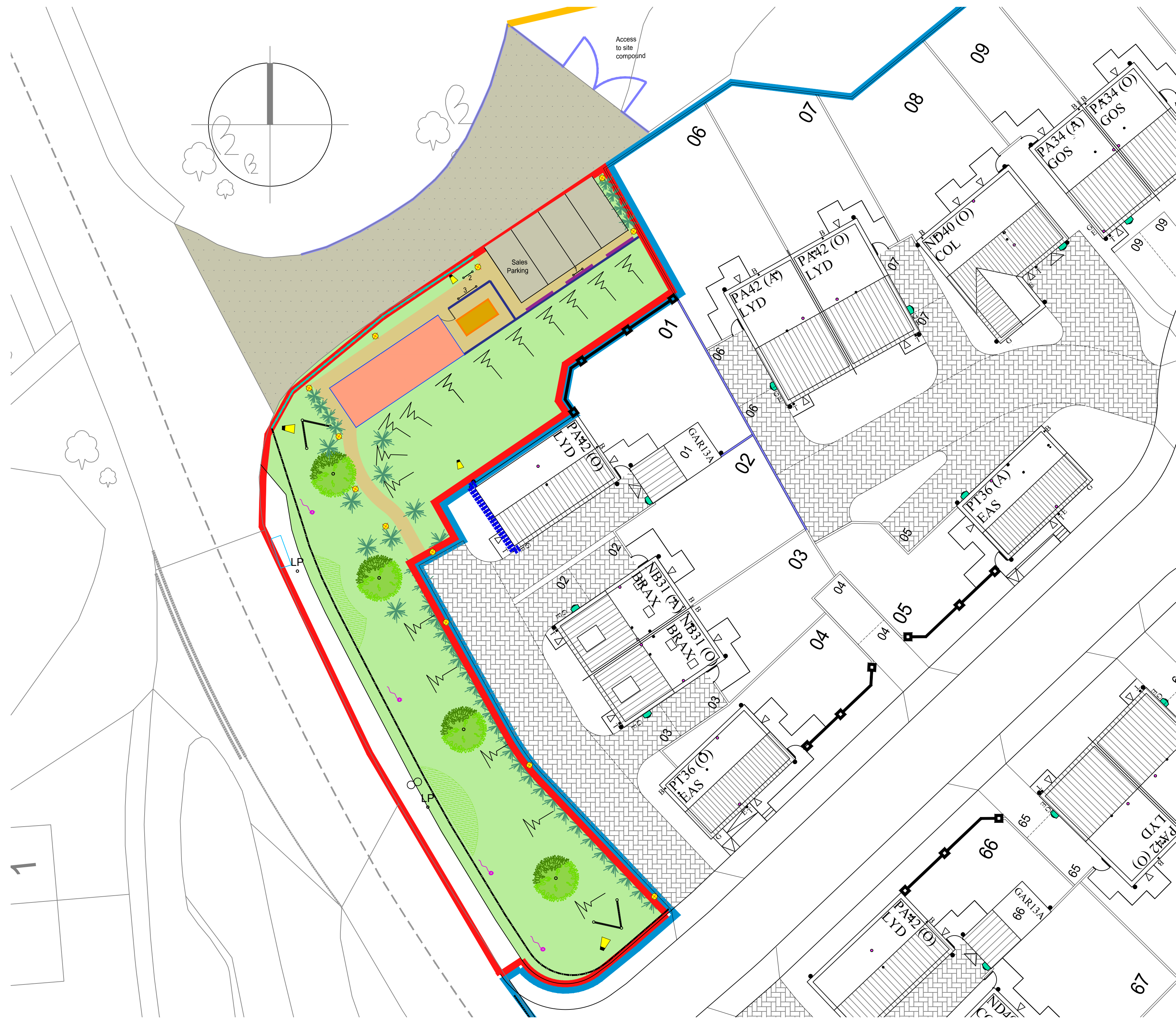
Plan drawing scale 1:200
