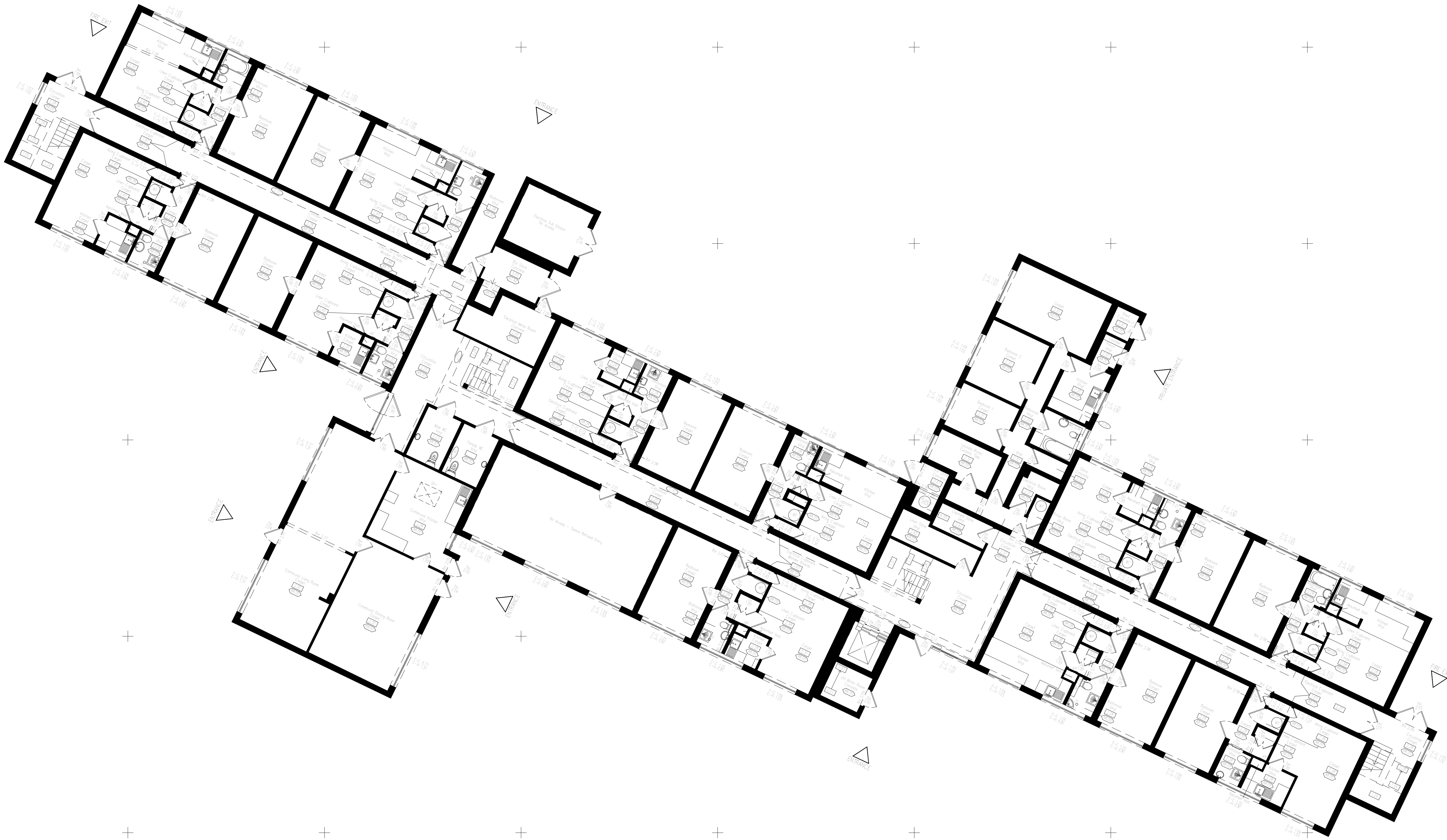
1 | Level 00 As Existing (Building Survey)
