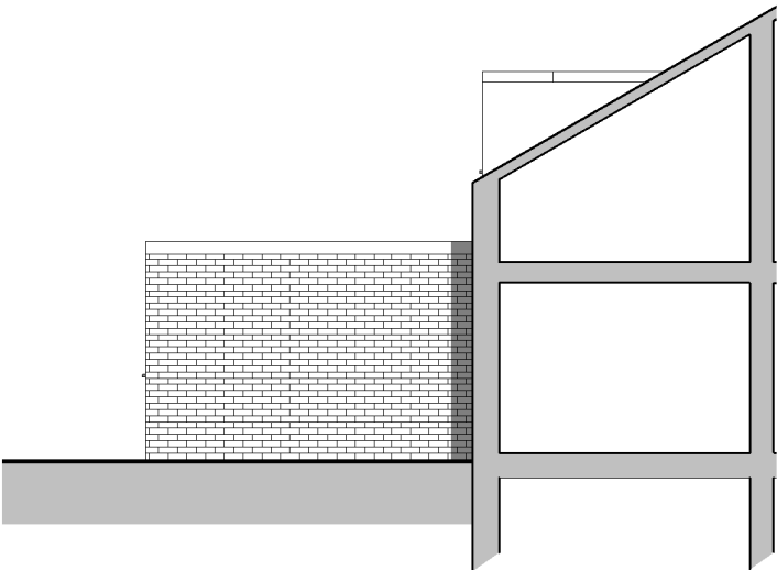
Side Elevation 1 : 100
