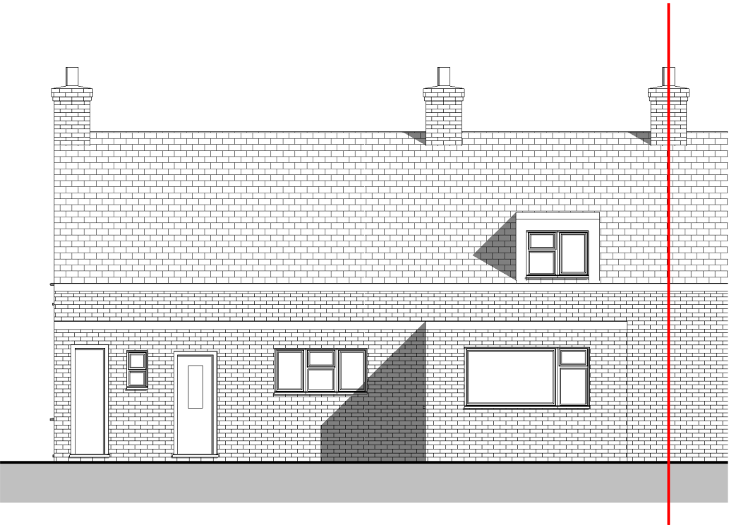
Rear Elevation 1 : 100
