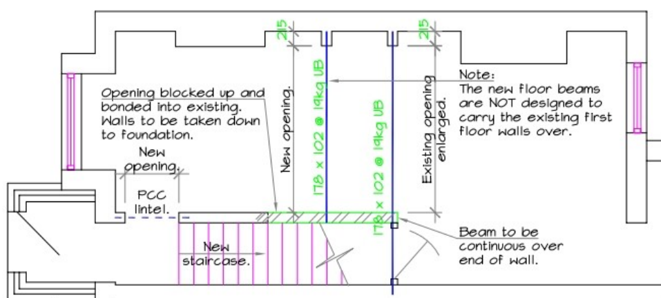
INDICATIVE FIRST FLOOR PLAN
