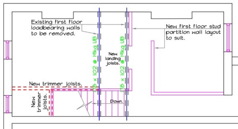
INDICATIVE FIRST FLOOR PLAN
