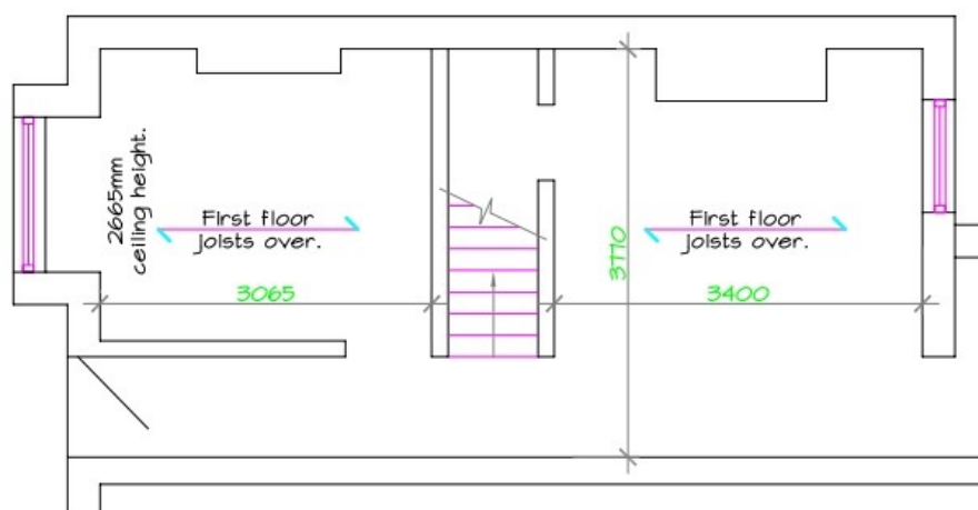
INDICATIVE EXISTING GROUND FLOOR PLAN
